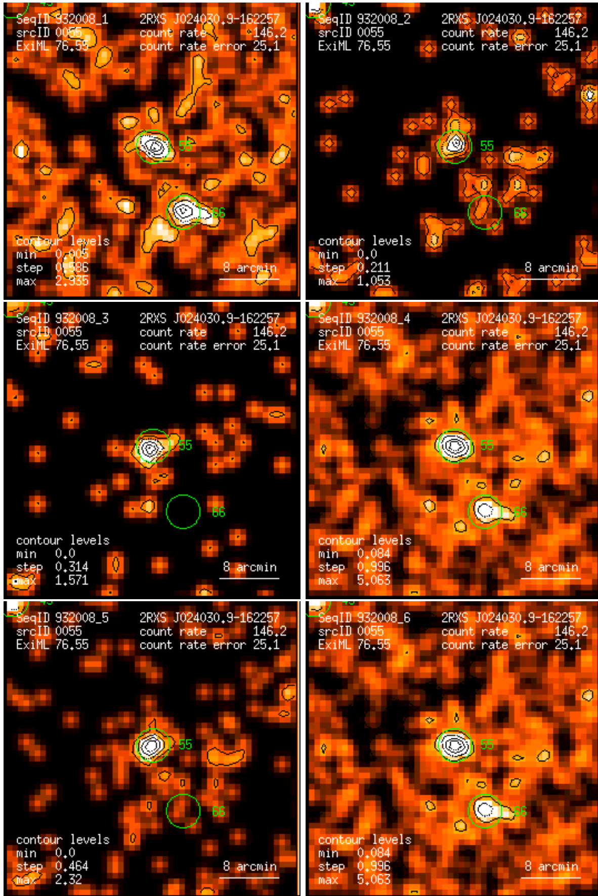
Figure 55: RASS 932008: detection 0055: band rate images, Gaussian filter: (1) PSPC channels 11 – 41, (2) 52 – 90, (3) 91 – 201, (4) 11 – 235, (5) 52 – 201, (6) 11 – 201. Broad band rates in counts/ks. Band rate contour levels in counts/ks/arcmin 2 .
