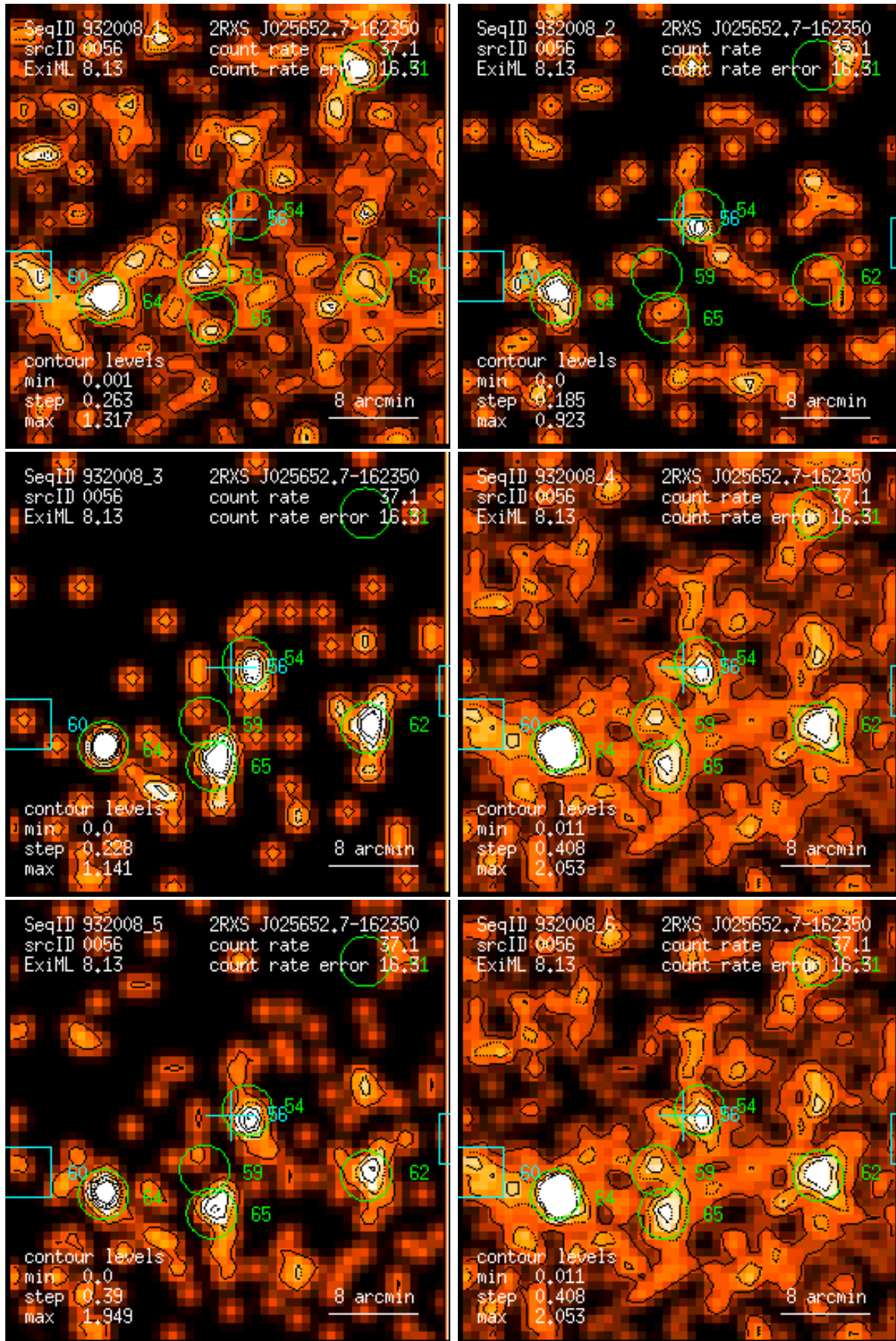
Figure 56: RASS 932008: detection 0056: band rate images, Gaussian filter: (1) PSPC channels 11 – 41, (2) 52 – 90, (3) 91 – 201, (4) 11 – 235, (5) 52 – 201, (6) 11 – 201. Broad band rates in counts/ks. Band rate contour levels in counts/ks/arcmin 2 .
