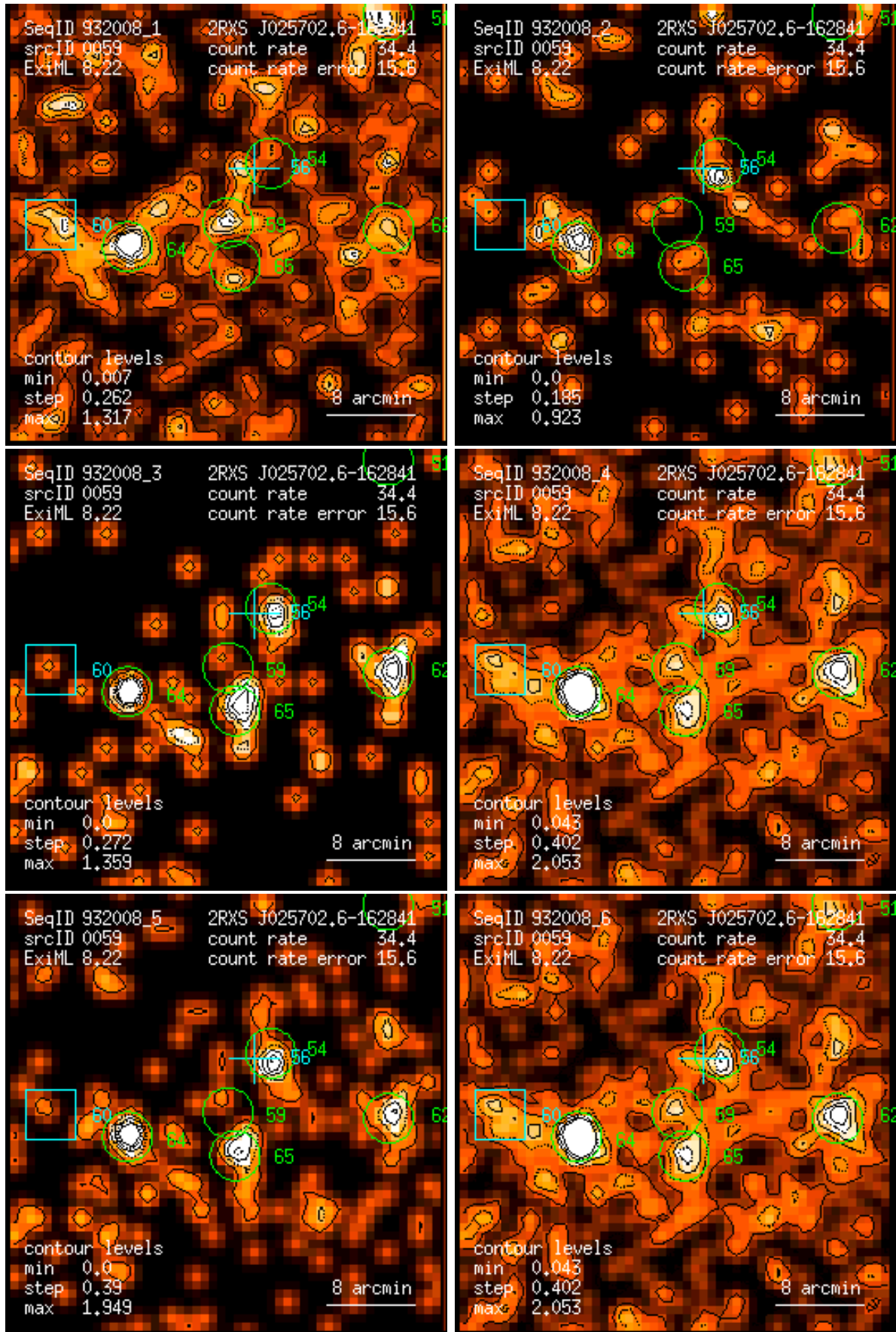
Figure 59: RASS 932008: detection 0059: band rate images, Gaussian filter: (1) PSPC channels 11 – 41, (2) 52 – 90, (3) 91 – 201, (4) 11 – 235, (5) 52 – 201, (6) 11 – 201. Broad band rates in counts/ks. Band rate contour levels in counts/ks/arcmin 2 .
