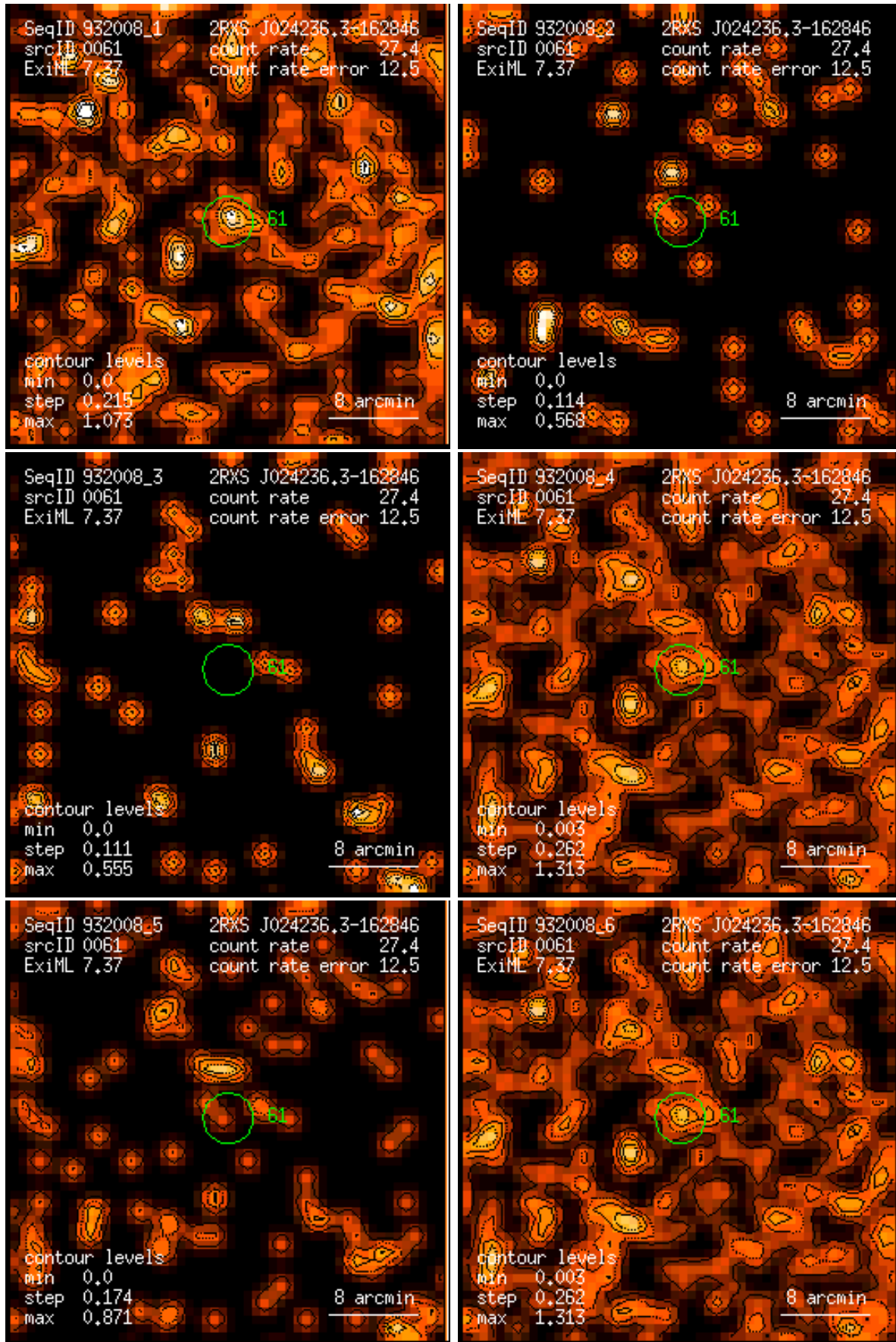
Figure 61: RASS 932008: detection 0061: band rate images, Gaussian filter: (1) PSPC channels 11 – 41, (2) 52 – 90, (3) 91 – 201, (4) 11 – 235, (5) 52 – 201, (6) 11 – 201. Broad band rates in counts/ks. Band rate contour levels in counts/ks/arcmin 2 .
