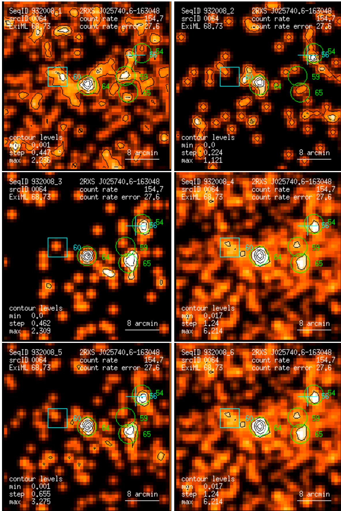
Figure 64: RASS 932008: detection 0064: band rate images, Gaussian filter: (1) PSPC channels 11 – 41, (2) 52 – 90, (3) 91 – 201, (4) 11 – 235, (5) 52 – 201, (6) 11 – 201. Broad band rates in counts/ks. Band rate contour levels in counts/ks/arcmin 2 .
