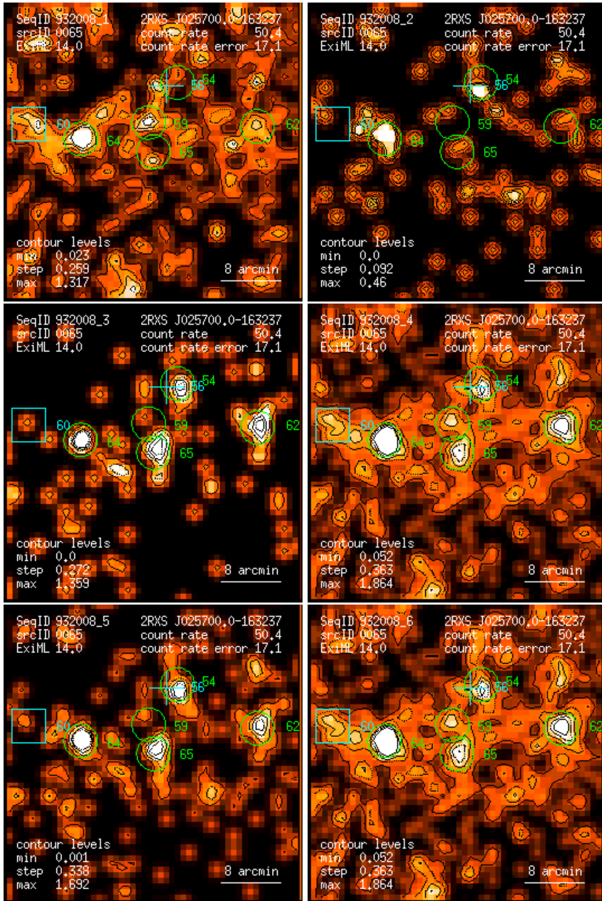
Figure 65: RASS 932008: detection 0065: band rate images, Gaussian filter: (1) PSPC channels 11 – 41, (2) 52 – 90, (3) 91 – 201, (4) 11 – 235, (5) 52 – 201, (6) 11 – 201. Broad band rates in counts/ks. Band rate contour levels in counts/ks/arcmin 2 .
