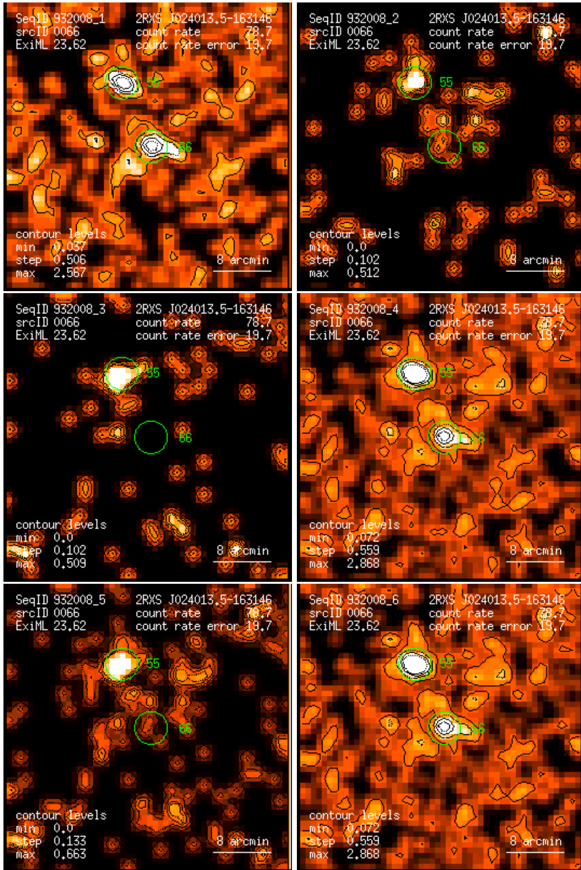
Figure 66: RASS 932008: detection 0066: band rate images, Gaussian filter: (1) PSPC channels 11 – 41, (2) 52 – 90, (3) 91 – 201, (4) 11 – 235, (5) 52 – 201, (6) 11 – 201. Broad band rates in counts/ks. Band rate contour levels in counts/ks/arcmin 2 .
