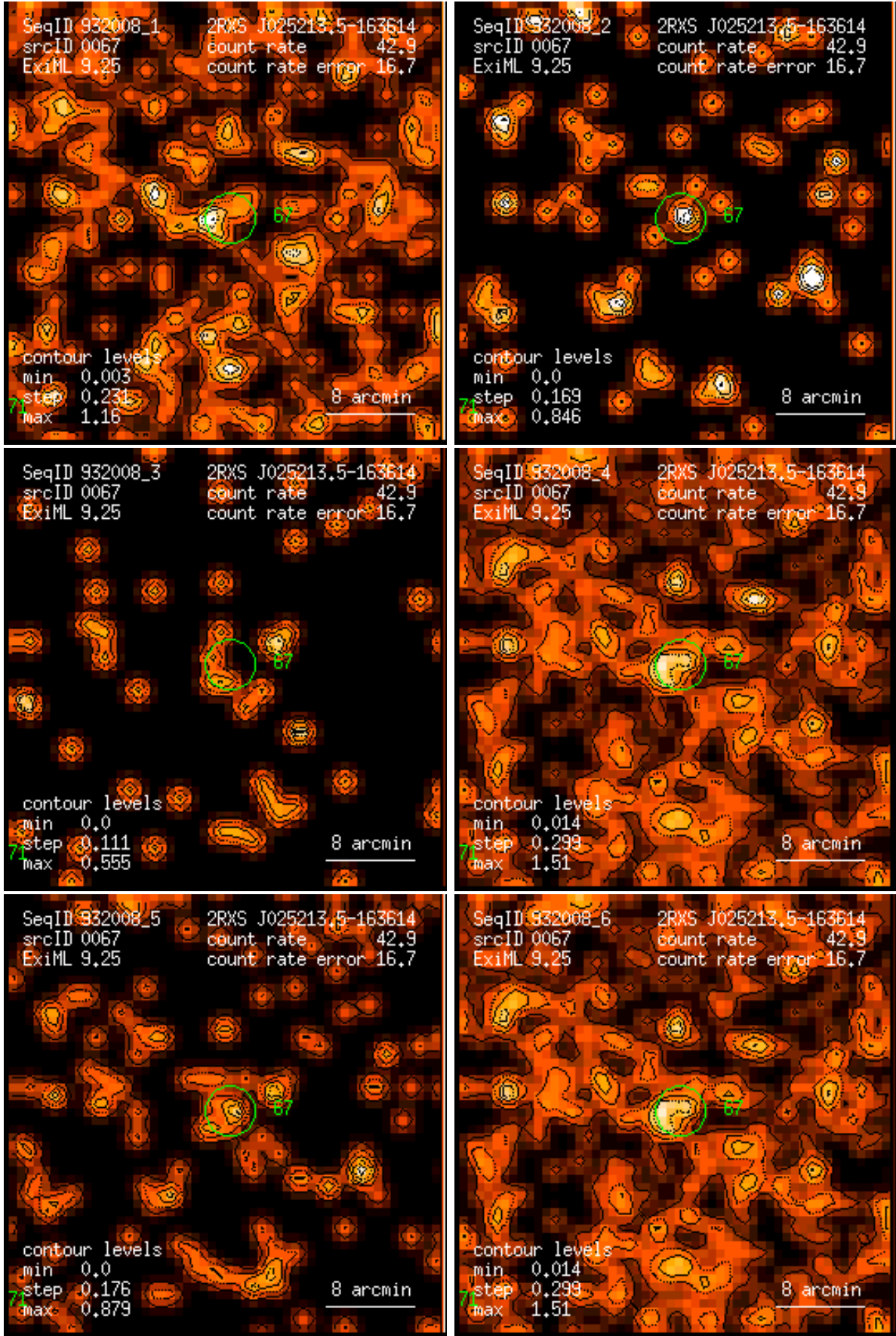
Figure 67: RASS 932008: detection 0067: band rate images, Gaussian filter: (1) PSPC channels 11 – 41, (2) 52 – 90, (3) 91 – 201, (4) 11 – 235, (5) 52 – 201, (6) 11 – 201. Broad band rates in counts/ks. Band rate contour levels in counts/ks/arcmin 2 .
