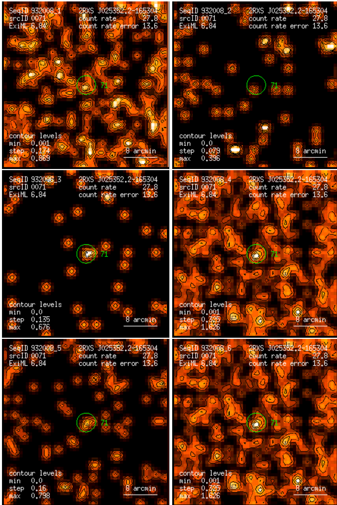
Figure 71: RASS 932008: detection 0071: band rate images, Gaussian filter: (1) PSPC channels 11 – 41, (2) 52 – 90, (3) 91 – 201, (4) 11 – 235, (5) 52 – 201, (6) 11 – 201. Broad band rates in counts/ks. Band rate contour levels in counts/ks/arcmin 2 .
