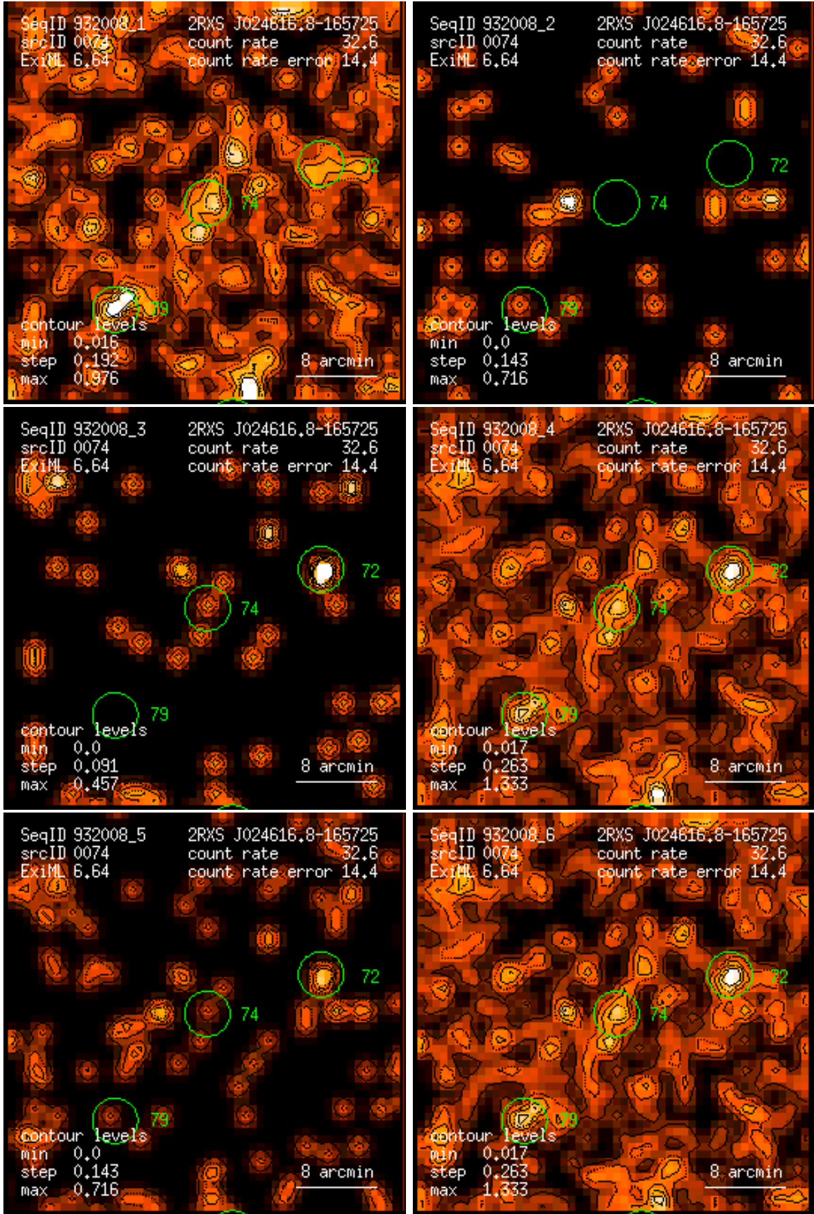
Figure 74: RASS 932008: detection 0074: band rate images, Gaussian filter: (1) PSPC channels 11 – 41, (2) 52 – 90, (3) 91 – 201, (4) 11 – 235, (5) 52 – 201, (6) 11 – 201. Broad band rates in counts/ks. Band rate contour levels in counts/ks/arcmin 2 .
