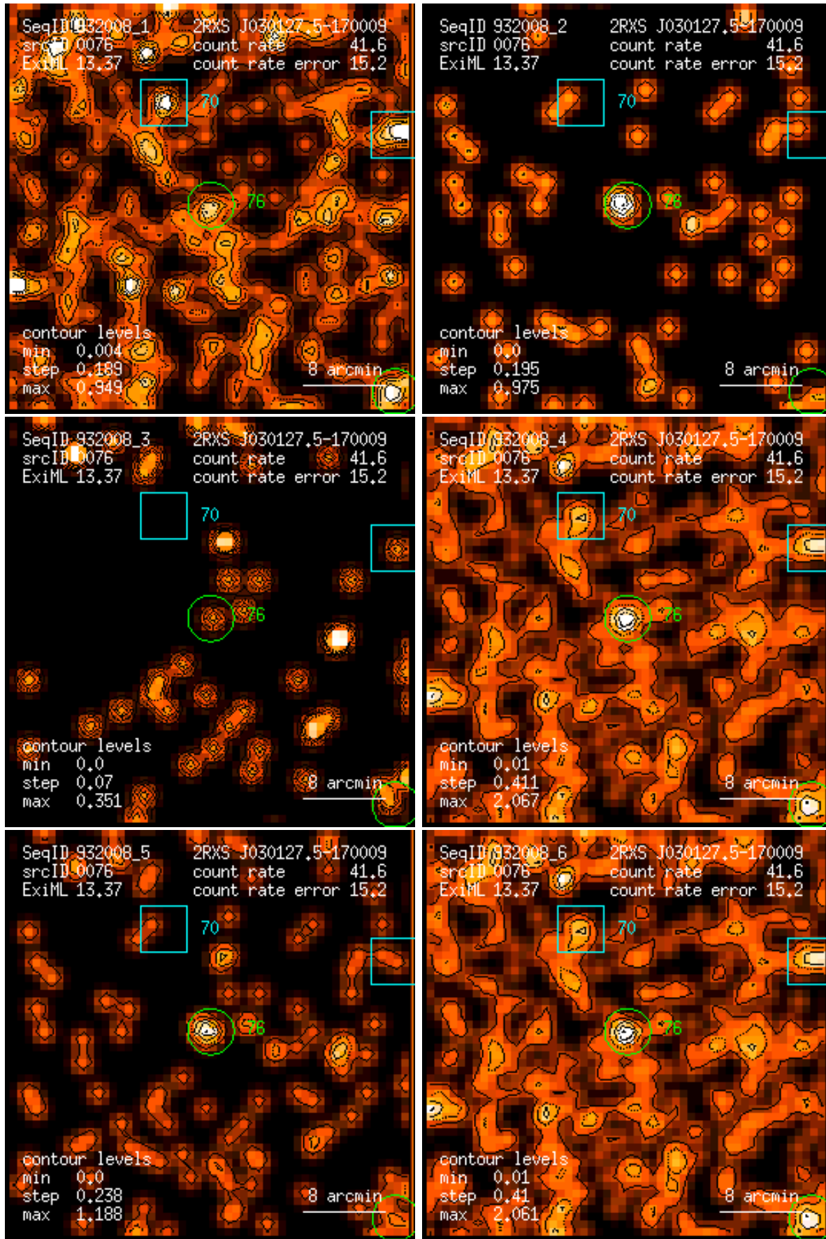
Figure 76: RASS 932008: detection 0076: band rate images, Gaussian filter: (1) PSPC channels 11 – 41, (2) 52 – 90, (3) 91 – 201, (4) 11 – 235, (5) 52 – 201, (6) 11 – 201. Broad band rates in counts/ks. Band rate contour levels in counts/ks/arcmin 2 .
