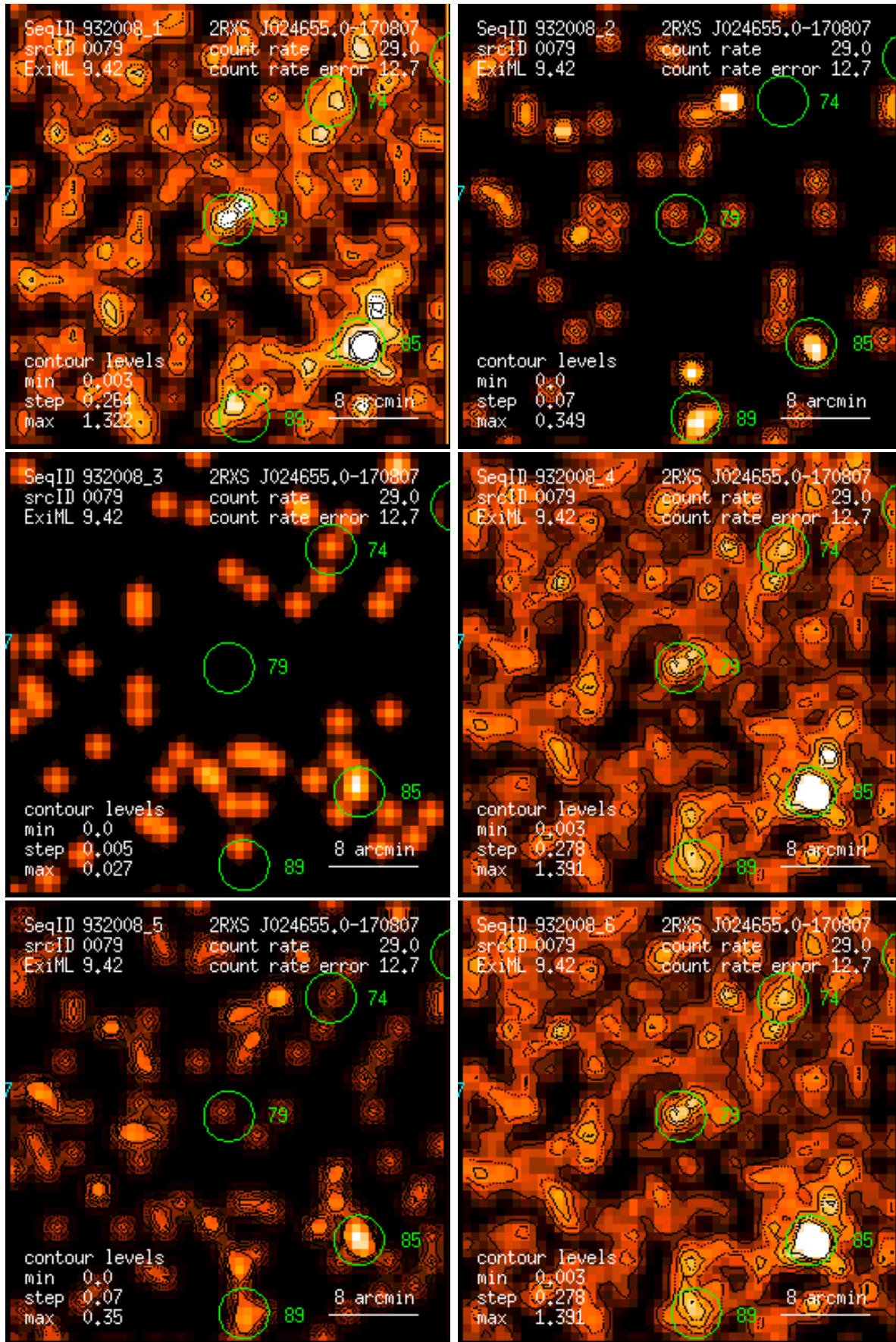
Figure 79: RASS 932008: detection 0079: band rate images, Gaussian filter: (1) PSPC channels 11 – 41, (2) 52 – 90, (3) 91 – 201, (4) 11 – 235, (5) 52 – 201, (6) 11 – 201. Broad band rates in counts/ks. Band rate contour levels in counts/ks/arcmin 2 .
