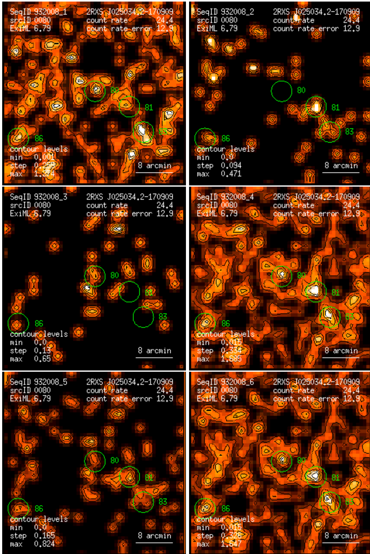
Figure 80: RASS 932008: detection 0080: band rate images, Gaussian filter: (1) PSPC channels 11 – 41, (2) 52 – 90, (3) 91 – 201, (4) 11 – 235, (5) 52 – 201, (6) 11 – 201. Broad band rates in counts/ks. Band rate contour levels in counts/ks/arcmin 2 .
