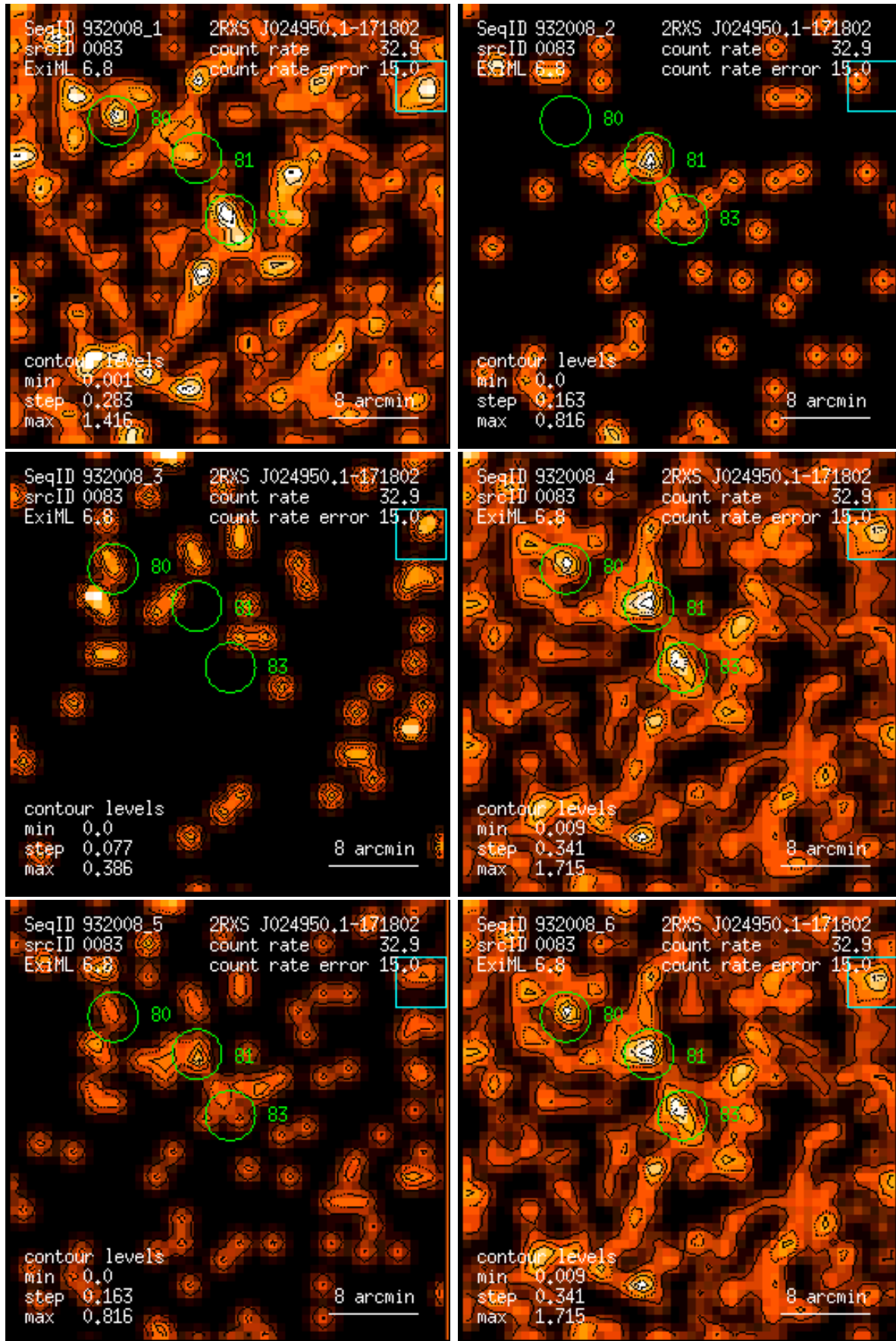
Figure 83: RASS 932008: detection 0083: band rate images, Gaussian filter: (1) PSPC channels 11 – 41, (2) 52 – 90, (3) 91 – 201, (4) 11 – 235, (5) 52 – 201, (6) 11 – 201. Broad band rates in counts/ks. Band rate contour levels in counts/ks/arcmin 2 .
