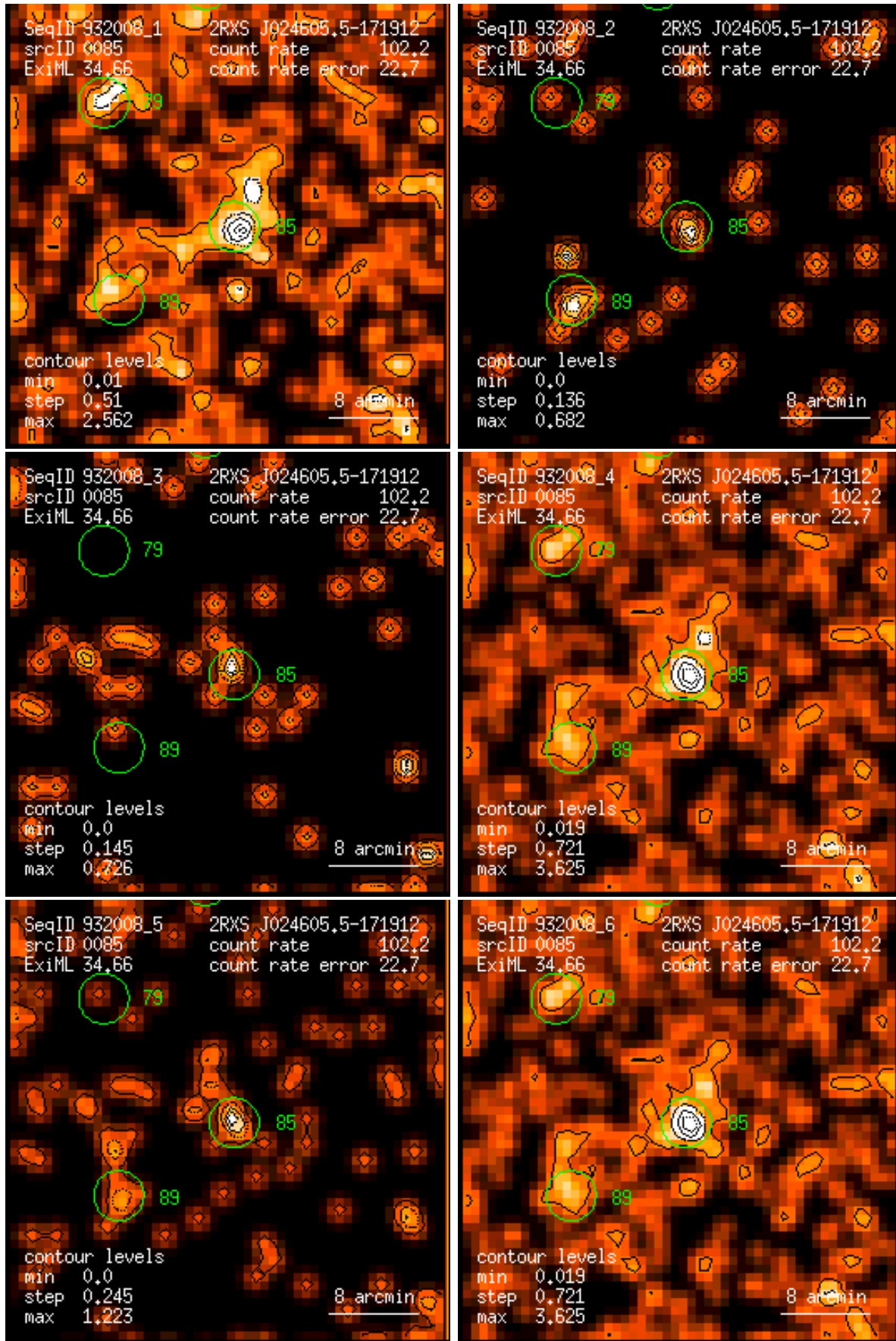
Figure 85: RASS 932008: detection 0085: band rate images, Gaussian filter: (1) PSPC channels 11 – 41, (2) 52 – 90, (3) 91 – 201, (4) 11 – 235, (5) 52 – 201, (6) 11 – 201. Broad band rates in counts/ks. Band rate contour levels in counts/ks/arcmin 2 .
