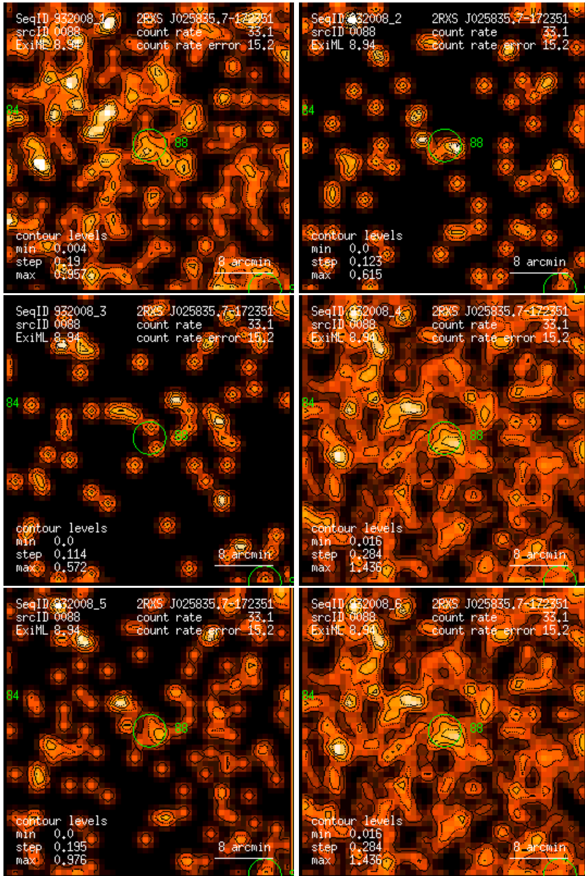
Figure 88: RASS 932008: detection 0088: band rate images, Gaussian filter: (1) PSPC channels 11 – 41, (2) 52 – 90, (3) 91 – 201, (4) 11 – 235, (5) 52 – 201, (6) 11 – 201. Broad band rates in counts/ks. Band rate contour levels in counts/ks/arcmin 2 .
