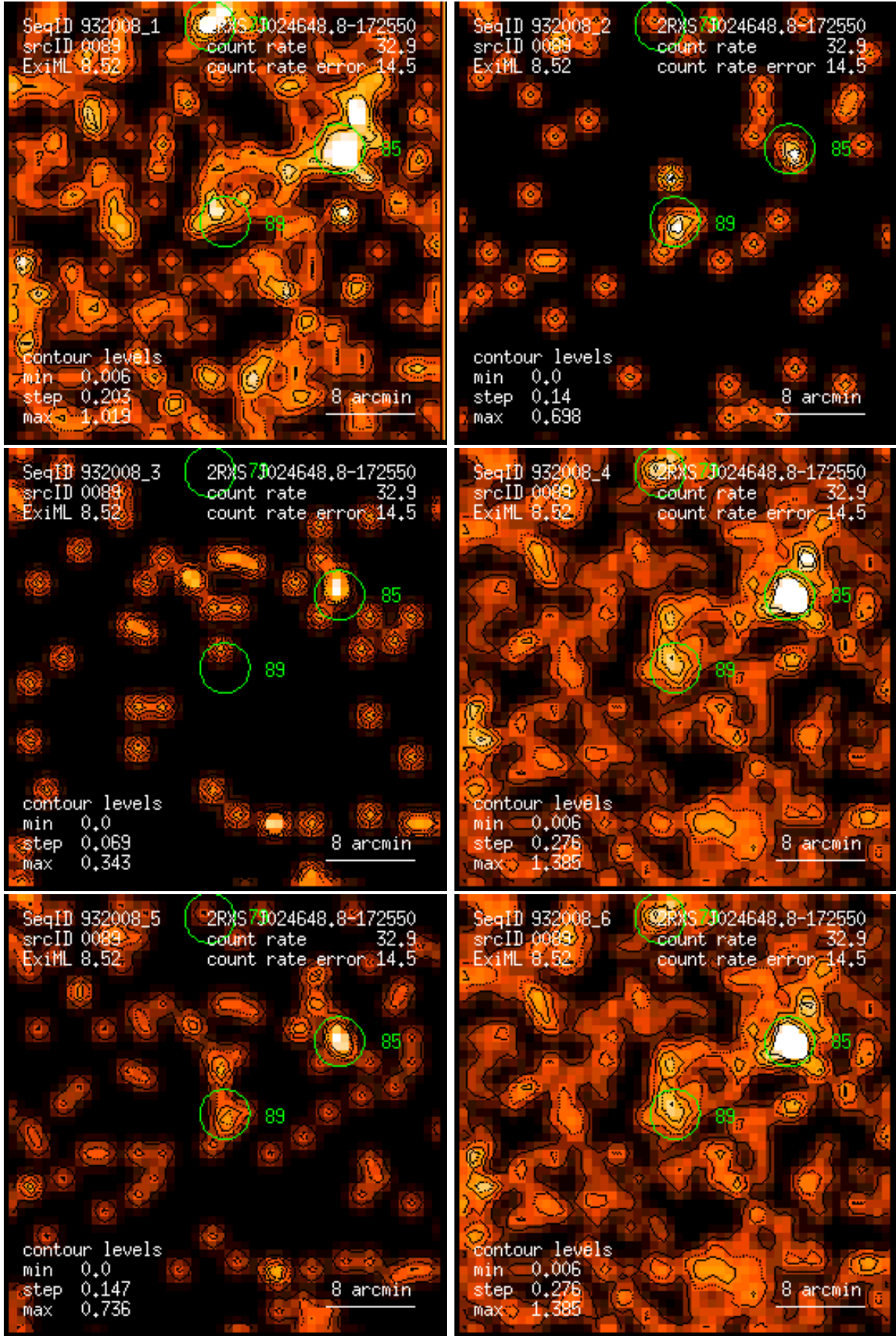
Figure 89: RASS 932008: detection 0089: band rate images, Gaussian filter: (1) PSPC channels 11 – 41, (2) 52 – 90, (3) 91 – 201, (4) 11 – 235, (5) 52 – 201, (6) 11 – 201. Broad band rates in counts/ks. Band rate contour levels in counts/ks/arcmin 2 .
