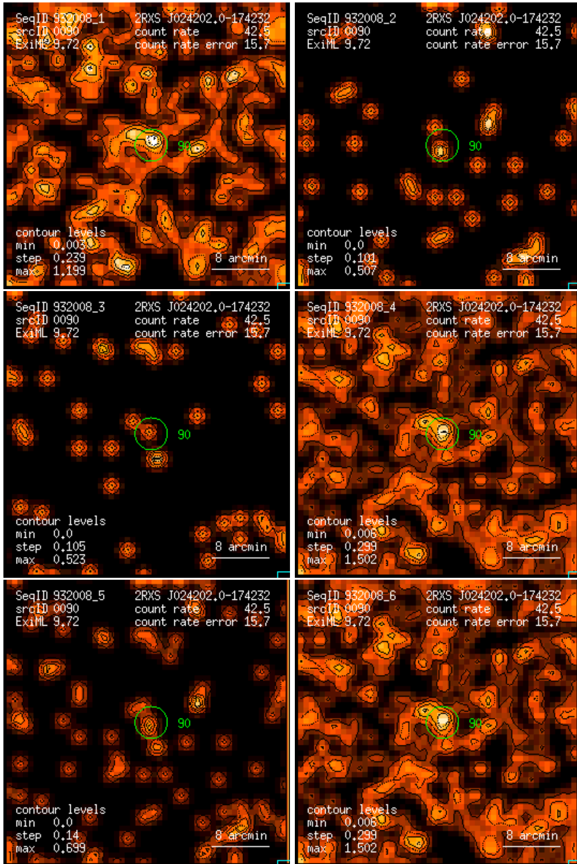
Figure 90: RASS 932008: detection 0090: band rate images, Gaussian filter: (1) PSPC channels 11 – 41, (2) 52 – 90, (3) 91 – 201, (4) 11 – 235, (5) 52 – 201, (6) 11 – 201. Broad band rates in counts/ks. Band rate contour levels in counts/ks/arcmin 2 .
