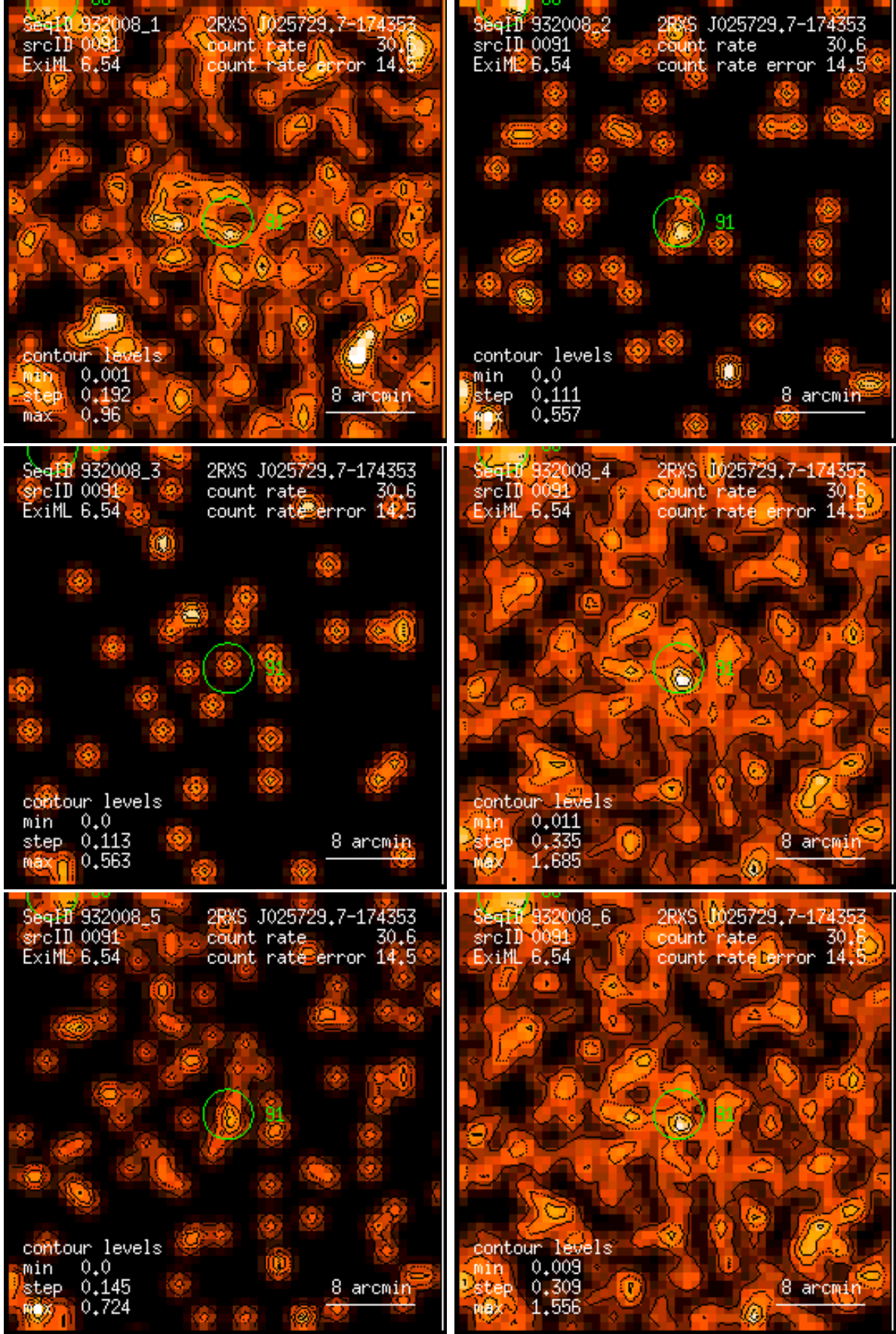
Figure 91: RASS 932008: detection 0091: band rate images, Gaussian filter: (1) PSPC channels 11 – 41, (2) 52 – 90, (3) 91 – 201, (4) 11 – 235, (5) 52 – 201, (6) 11 – 201. Broad band rates in counts/ks. Band rate contour levels in counts/ks/arcmin 2 .
