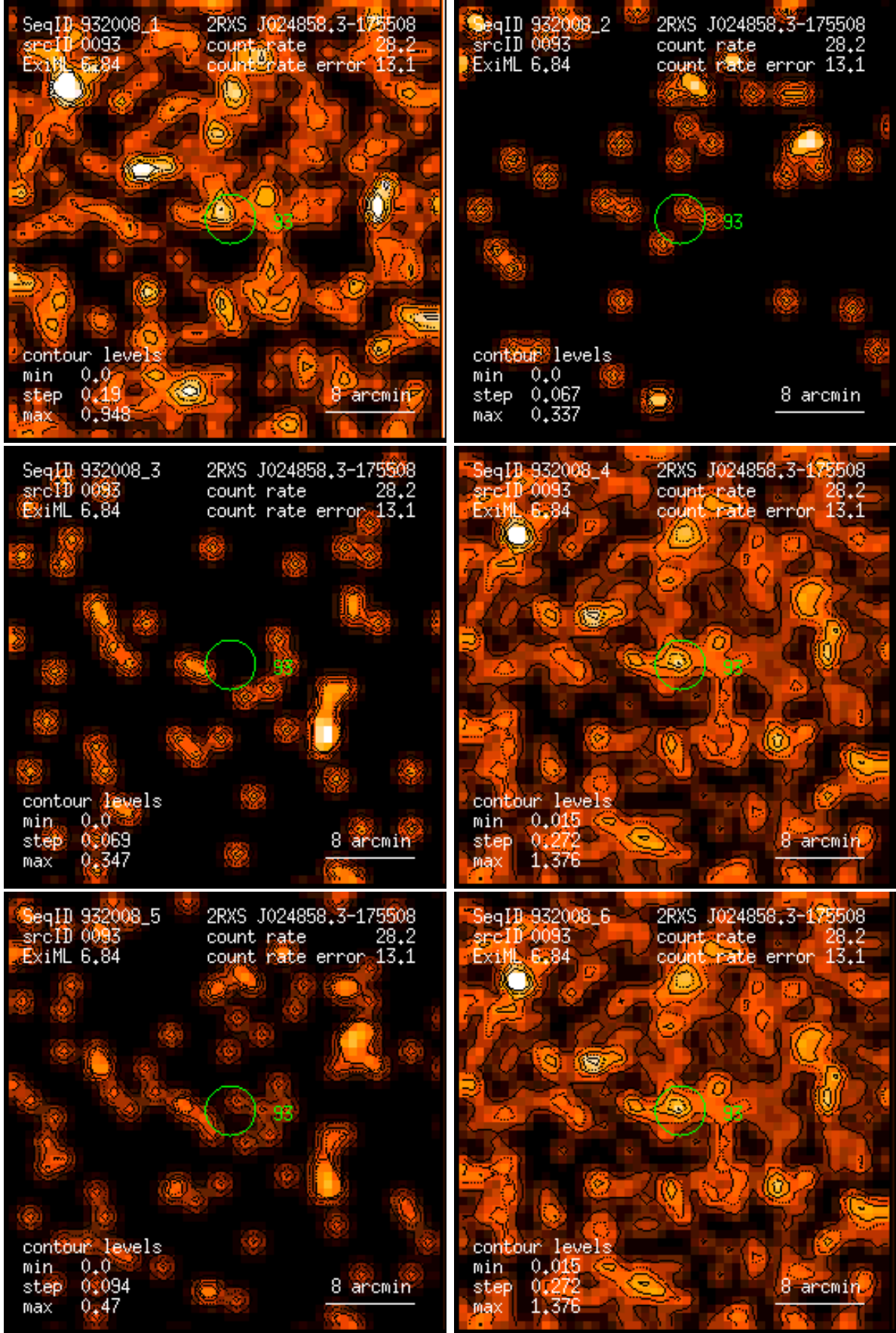
Figure 93: RASS 932008: detection 0093: band rate images, Gaussian filter: (1) PSPC channels 11 – 41, (2) 52 – 90, (3) 91 – 201, (4) 11 – 235, (5) 52 – 201, (6) 11 – 201. Broad band rates in counts/ks. Band rate contour levels in counts/ks/arcmin 2 .
