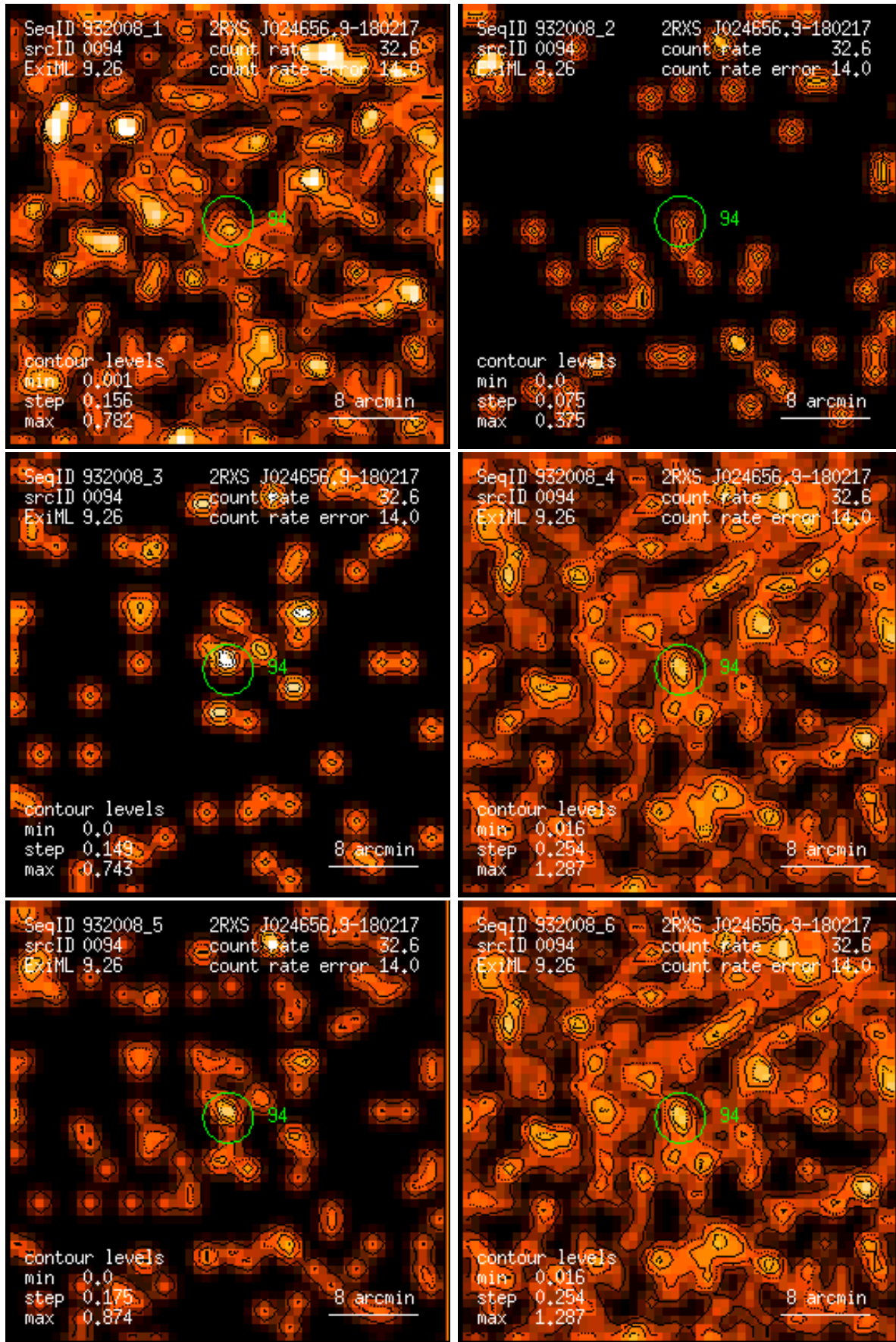
Figure 94: RASS 932008: detection 0094: band rate images, Gaussian filter: (1) PSPC channels 11 – 41, (2) 52 – 90, (3) 91 – 201, (4) 11 – 235, (5) 52 – 201, (6) 11 – 201. Broad band rates in counts/ks. Band rate contour levels in counts/ks/arcmin 2 .
