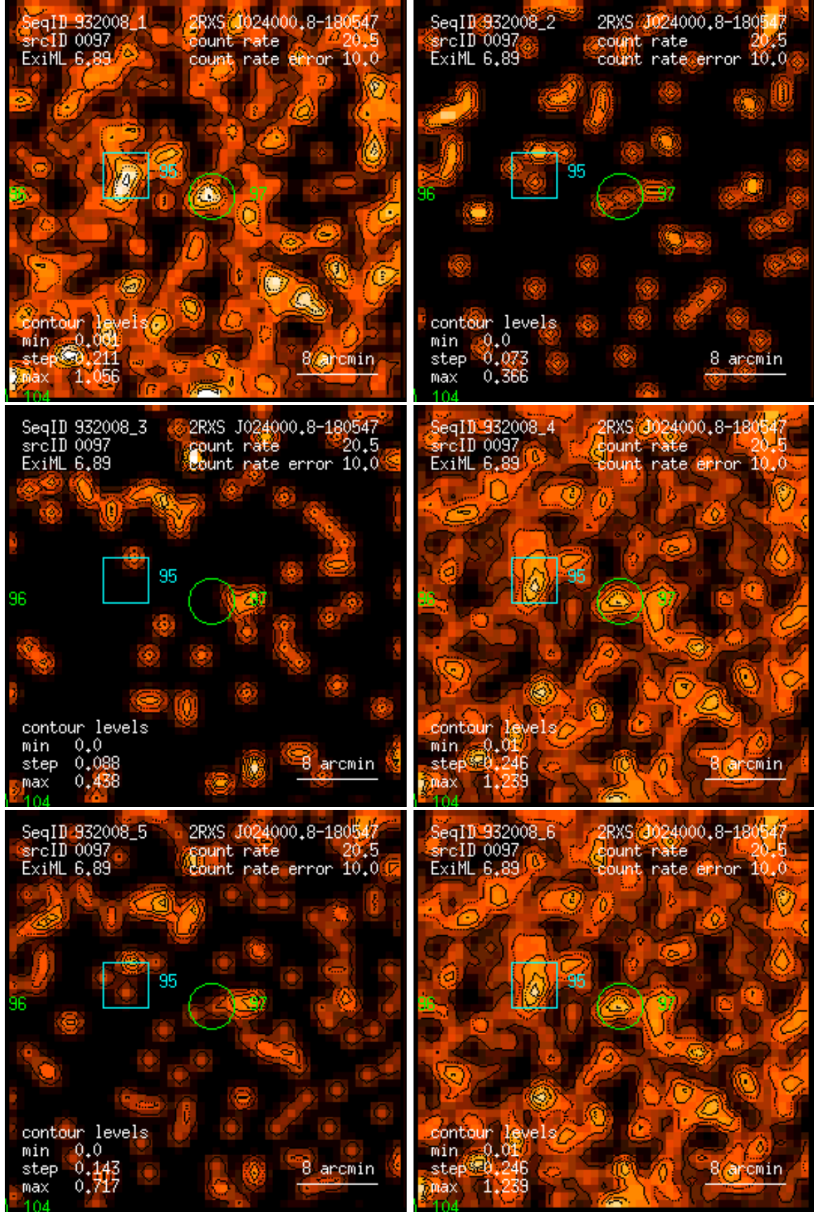
Figure 97: RASS 932008: detection 0097: band rate images, Gaussian filter: (1) PSPC channels 11 – 41, (2) 52 – 90, (3) 91 – 201, (4) 11 – 235, (5) 52 – 201, (6) 11 – 201. Broad band rates in counts/ks. Band rate contour levels in counts/ks/arcmin 2 .
