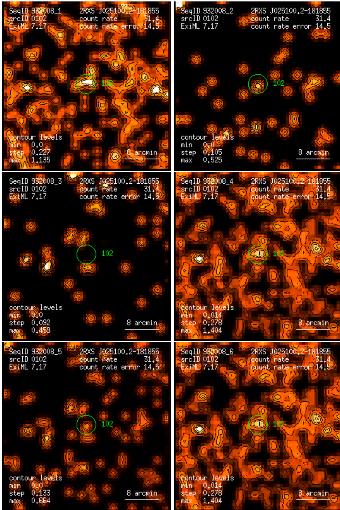
Figure 102: RASS 932008: detection 0102: band rate images, Gaussian filter: (1) PSPC channels 11 – 41, (2) 52 – 90, (3) 91 – 201, (4) 11 – 235, (5) 52 – 201, (6) 11 – 201. Broad band rates in counts/ks. Band rate contour levels in counts/ks/arcmin 2 .
