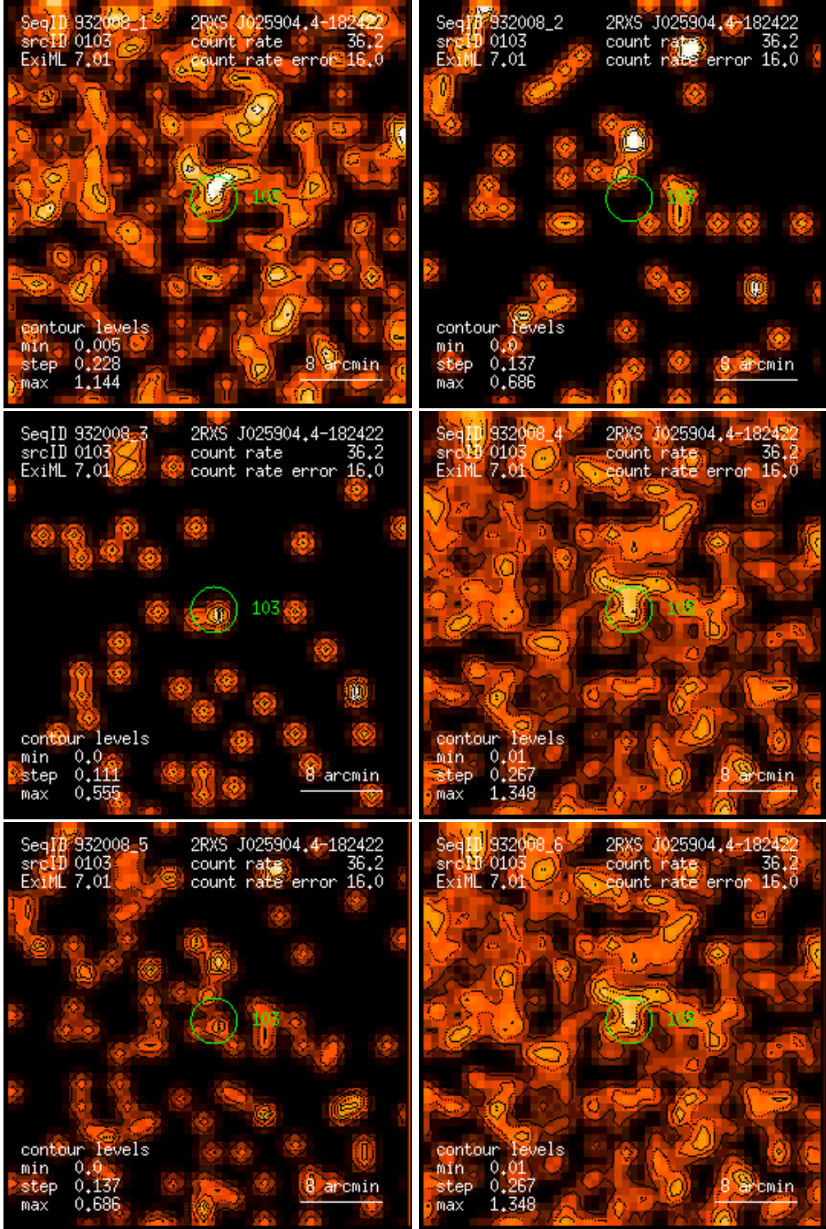
Figure 103: RASS 932008: detection 0103: band rate images, Gaussian filter: (1) PSPC channels 11 – 41, (2) 52 – 90, (3) 91 – 201, (4) 11 – 235, (5) 52 – 201, (6) 11 – 201. Broad band rates in counts/ks. Band rate contour levels in counts/ks/arcmin 2 .
