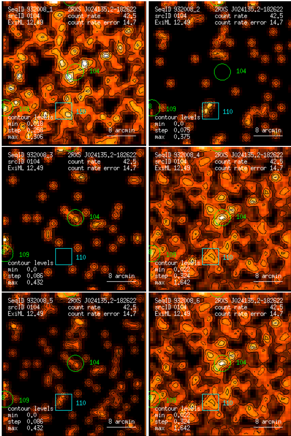
Figure 104: RASS 932008: detection 0104: band rate images, Gaussian filter: (1) PSPC channels 11 – 41, (2) 52 – 90, (3) 91 – 201, (4) 11 – 235, (5) 52 – 201, (6) 11 – 201. Broad band rates in counts/ks. Band rate contour levels in counts/ks/arcmin 2 .
