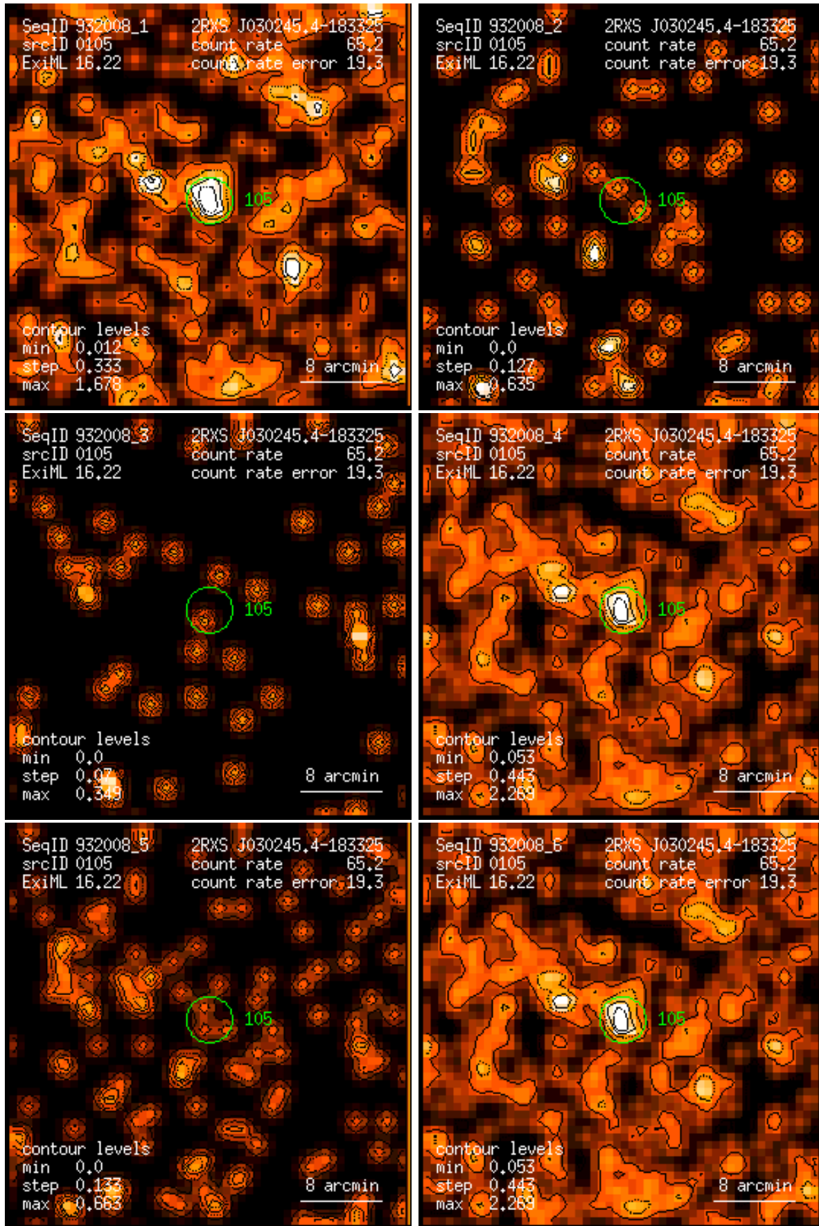
Figure 105: RASS 932008: detection 0105: band rate images, Gaussian filter: (1) PSPC channels 11 – 41, (2) 52 – 90, (3) 91 – 201, (4) 11 – 235, (5) 52 – 201, (6) 11 – 201. Broad band rates in counts/ks. Band rate contour levels in counts/ks/arcmin 2 .
