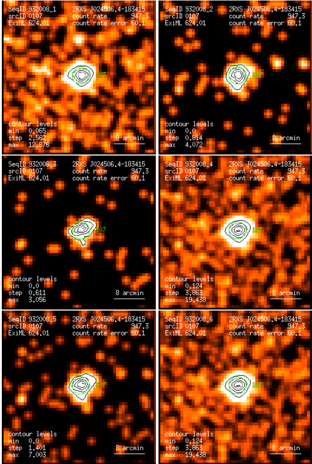
Figure 107: RASS 932008: detection 0107: band rate images, Gaussian filter: (1) PSPC channels 11 – 41, (2) 52 – 90, (3) 91 – 201, (4) 11 – 235, (5) 52 – 201, (6) 11 – 201. Broad band rates in counts/ks. Band rate contour levels in counts/ks/arcmin 2 .
