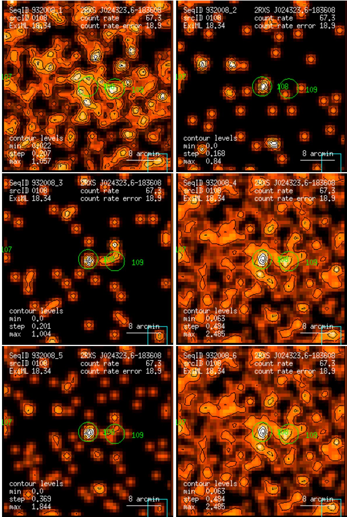
Figure 108: RASS 932008: detection 0108: band rate images, Gaussian filter: (1) PSPC channels 11 – 41, (2) 52 – 90, (3) 91 – 201, (4) 11 – 235, (5) 52 – 201, (6) 11 – 201. Broad band rates in counts/ks. Band rate contour levels in counts/ks/arcmin 2 .
