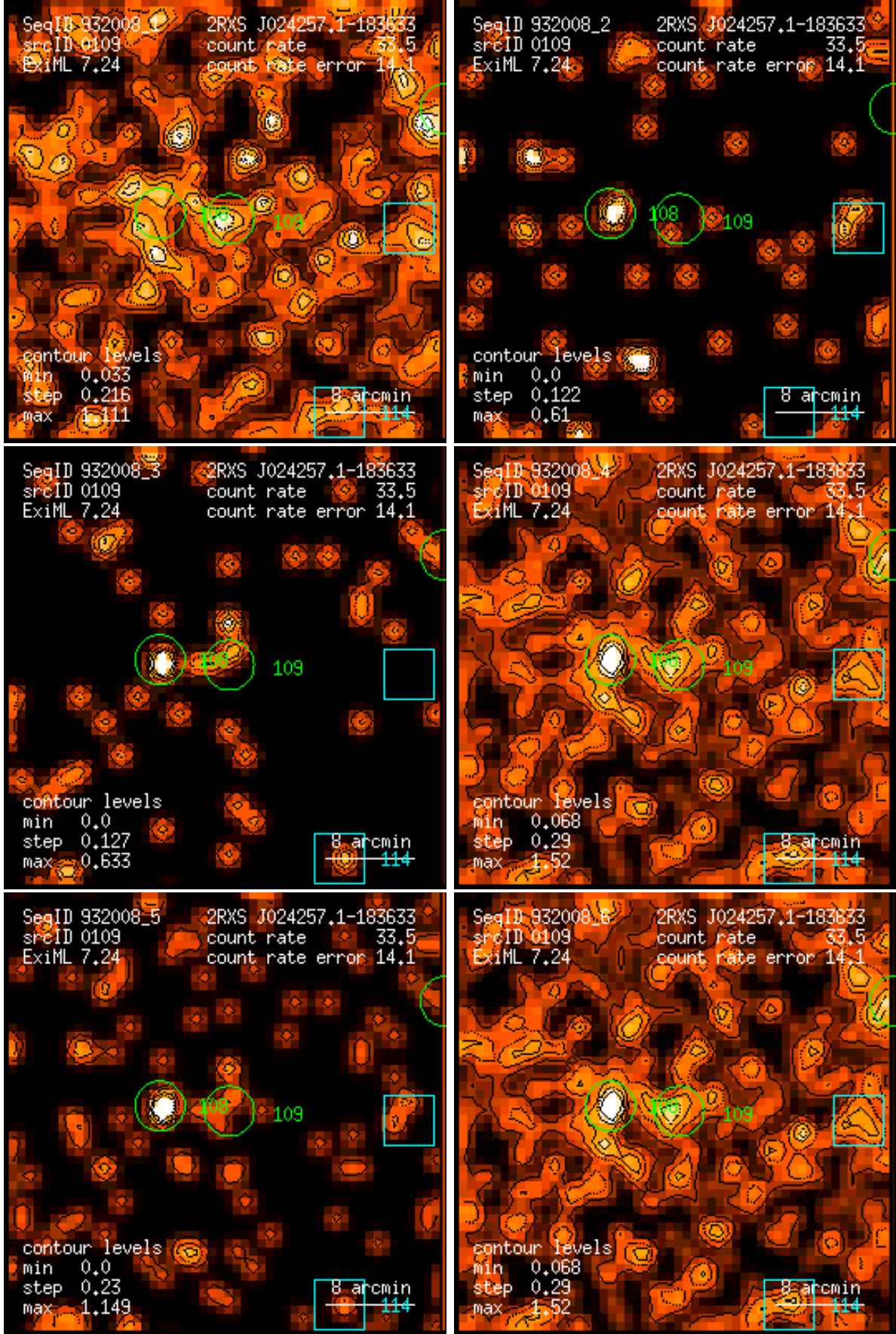
Figure 109: RASS 932008: detection 0109: band rate images, Gaussian filter: (1) PSPC channels 11 – 41, (2) 52 – 90, (3) 91 – 201, (4) 11 – 235, (5) 52 – 201, (6) 11 – 201. Broad band rates in counts/ks. Band rate contour levels in counts/ks/arcmin 2 .
