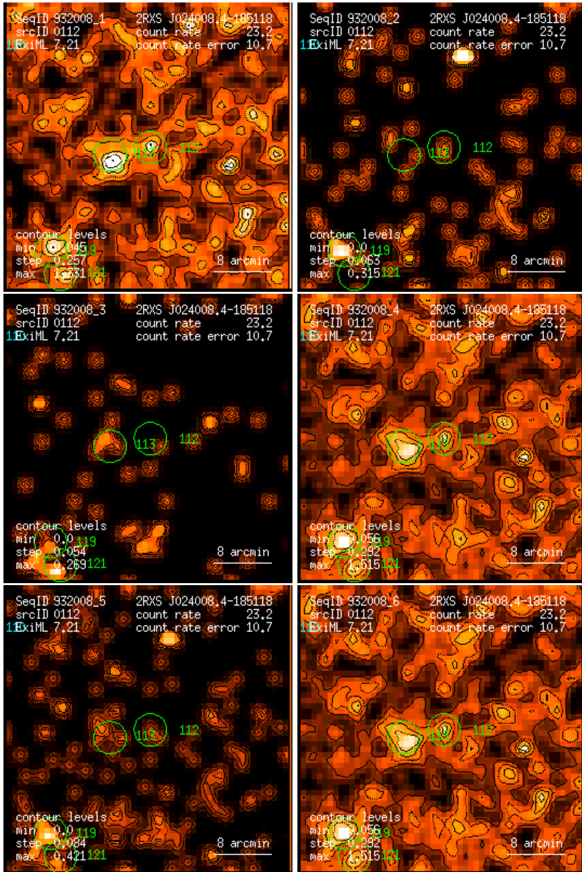
Figure 112: RASS 932008: detection 0112: band rate images, Gaussian filter: (1) PSPC channels 11 – 41, (2) 52 – 90, (3) 91 – 201, (4) 11 – 235, (5) 52 – 201, (6) 11 – 201. Broad band rates in counts/ks. Band rate contour levels in counts/ks/arcmin 2 .
