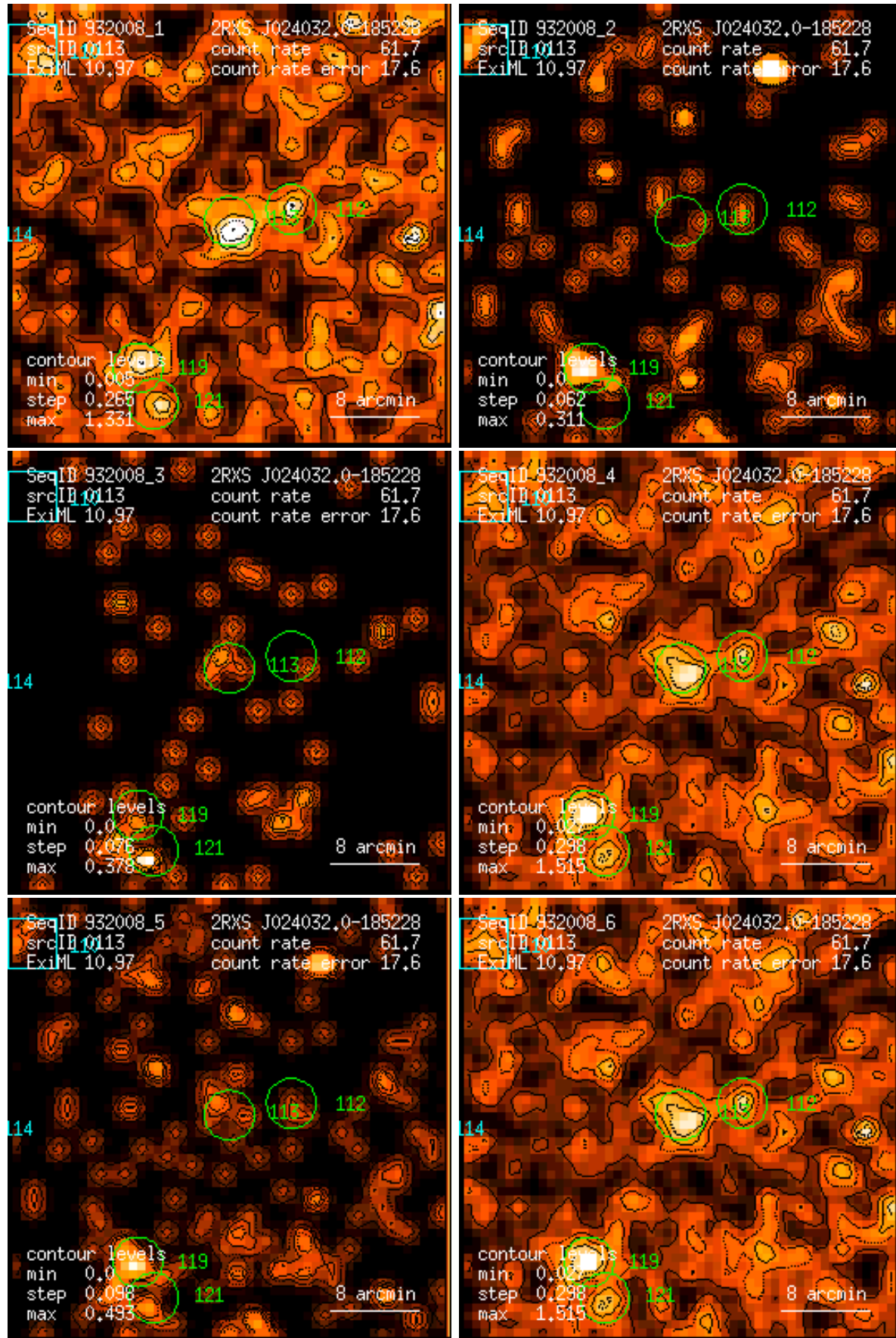
Figure 113: RASS 932008: detection 0113: band rate images, Gaussian filter: (1) PSPC channels 11 – 41, (2) 52 – 90, (3) 91 – 201, (4) 11 – 235, (5) 52 – 201, (6) 11 – 201. Broad band rates in counts/ks. Band rate contour levels in counts/ks/arcmin 2 .
