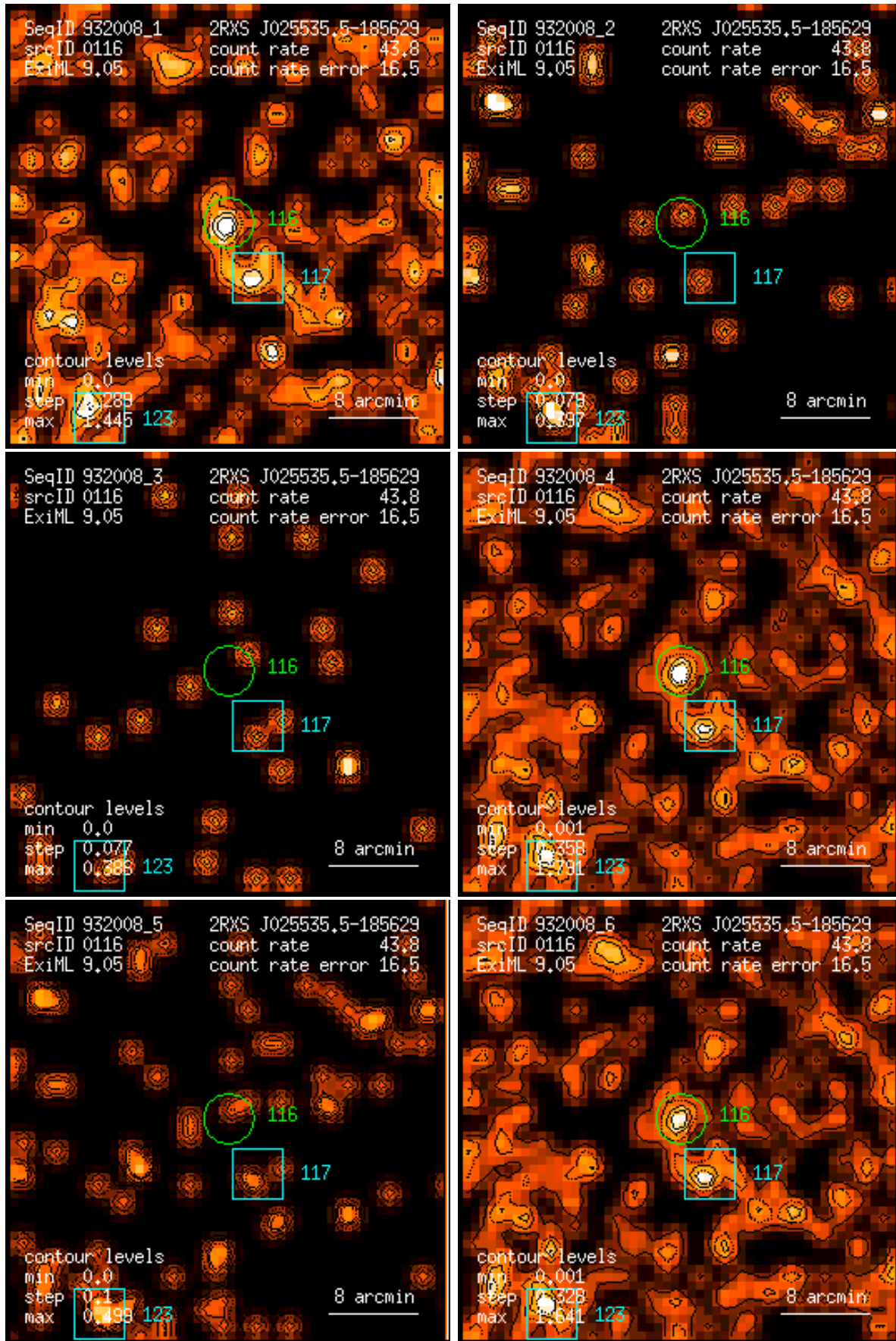
Figure 116: RASS 932008: detection 0116: band rate images, Gaussian filter: (1) PSPC channels 11 – 41, (2) 52 – 90, (3) 91 – 201, (4) 11 – 235, (5) 52 – 201, (6) 11 – 201. Broad band rates in counts/ks. Band rate contour levels in counts/ks/arcmin 2 .
