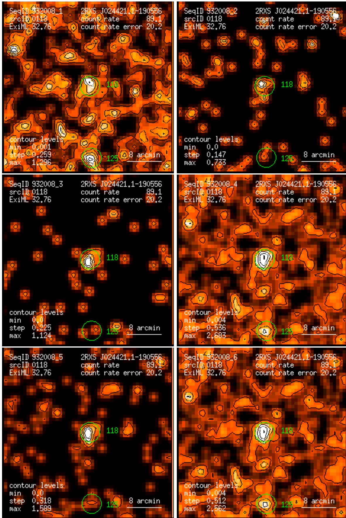
Figure 118: RASS 932008: detection 0118: band rate images, Gaussian filter: (1) PSPC channels 11 – 41, (2) 52 – 90, (3) 91 – 201, (4) 11 – 235, (5) 52 – 201, (6) 11 – 201. Broad band rates in counts/ks. Band rate contour levels in counts/ks/arcmin 2 .
