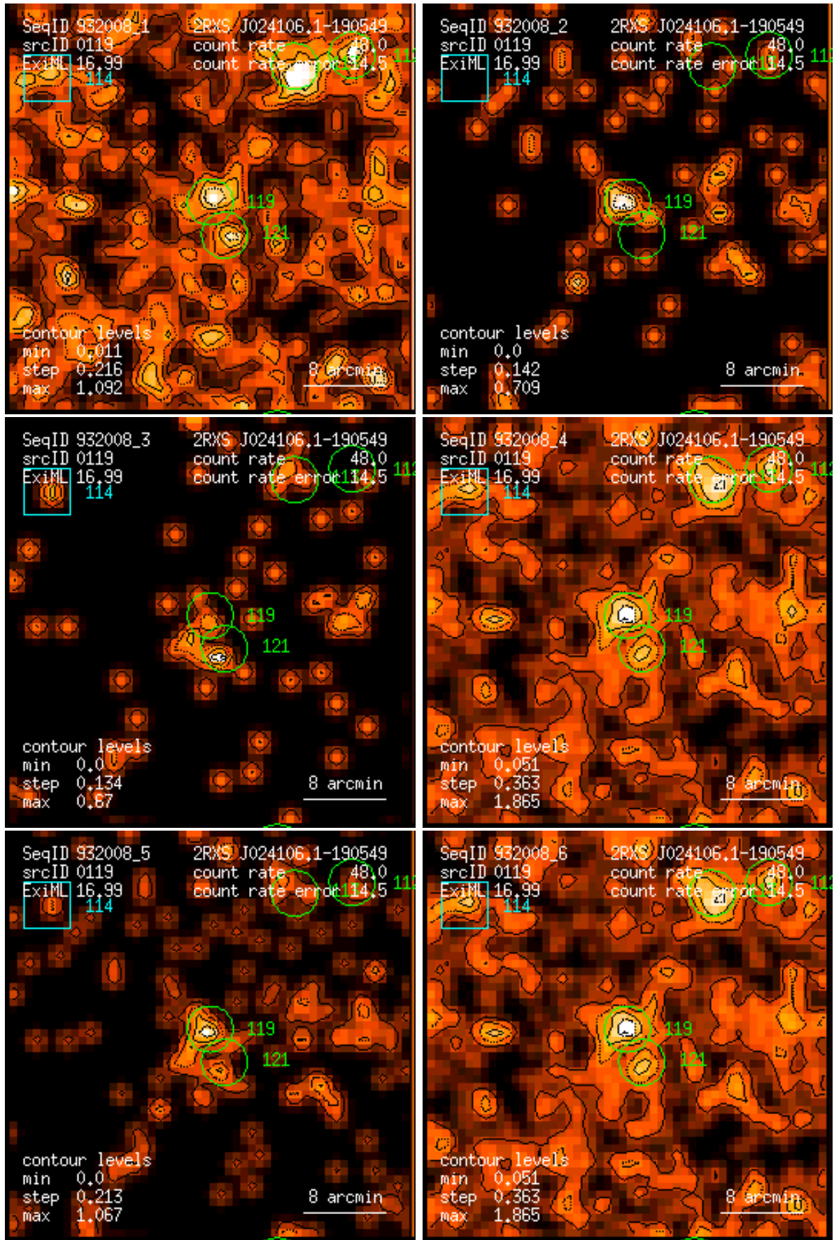
Figure 119: RASS 932008: detection 0119: band rate images, Gaussian filter: (1) PSPC channels 11 – 41, (2) 52 – 90, (3) 91 – 201, (4) 11 – 235, (5) 52 – 201, (6) 11 – 201. Broad band rates in counts/ks. Band rate contour levels in counts/ks/arcmin 2 .
