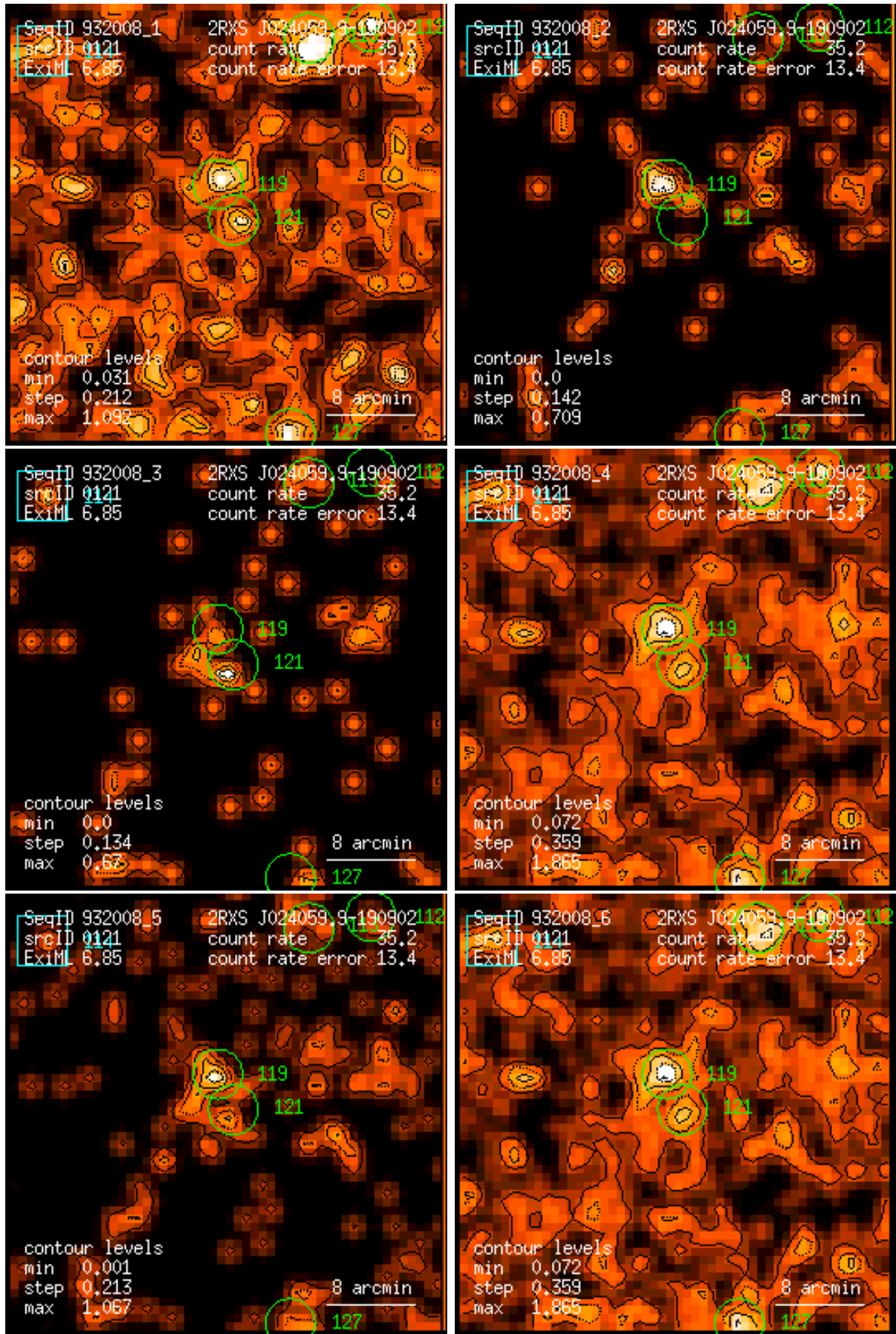
Figure 121: RASS 932008: detection 0121: band rate images, Gaussian filter: (1) PSPC channels 11 – 41, (2) 52 – 90, (3) 91 – 201, (4) 11 – 235, (5) 52 – 201, (6) 11 – 201. Broad band rates in counts/ks. Band rate contour levels in counts/ks/arcmin 2 .
