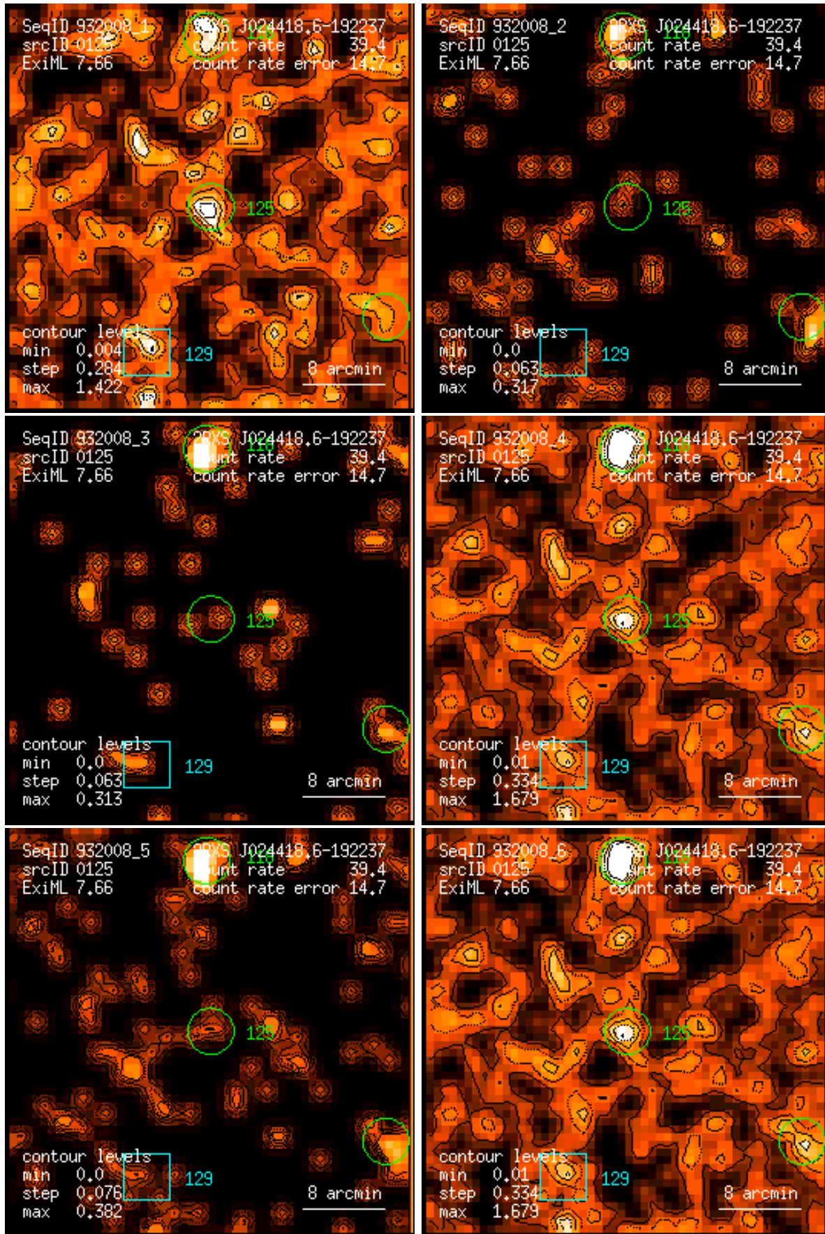
Figure 125: RASS 932008: detection 0125: band rate images, Gaussian filter: (1) PSPC channels 11 – 41, (2) 52 – 90, (3) 91 – 201, (4) 11 – 235, (5) 52 – 201, (6) 11 – 201. Broad band rates in counts/ks. Band rate contour levels in counts/ks/arcmin 2 .
