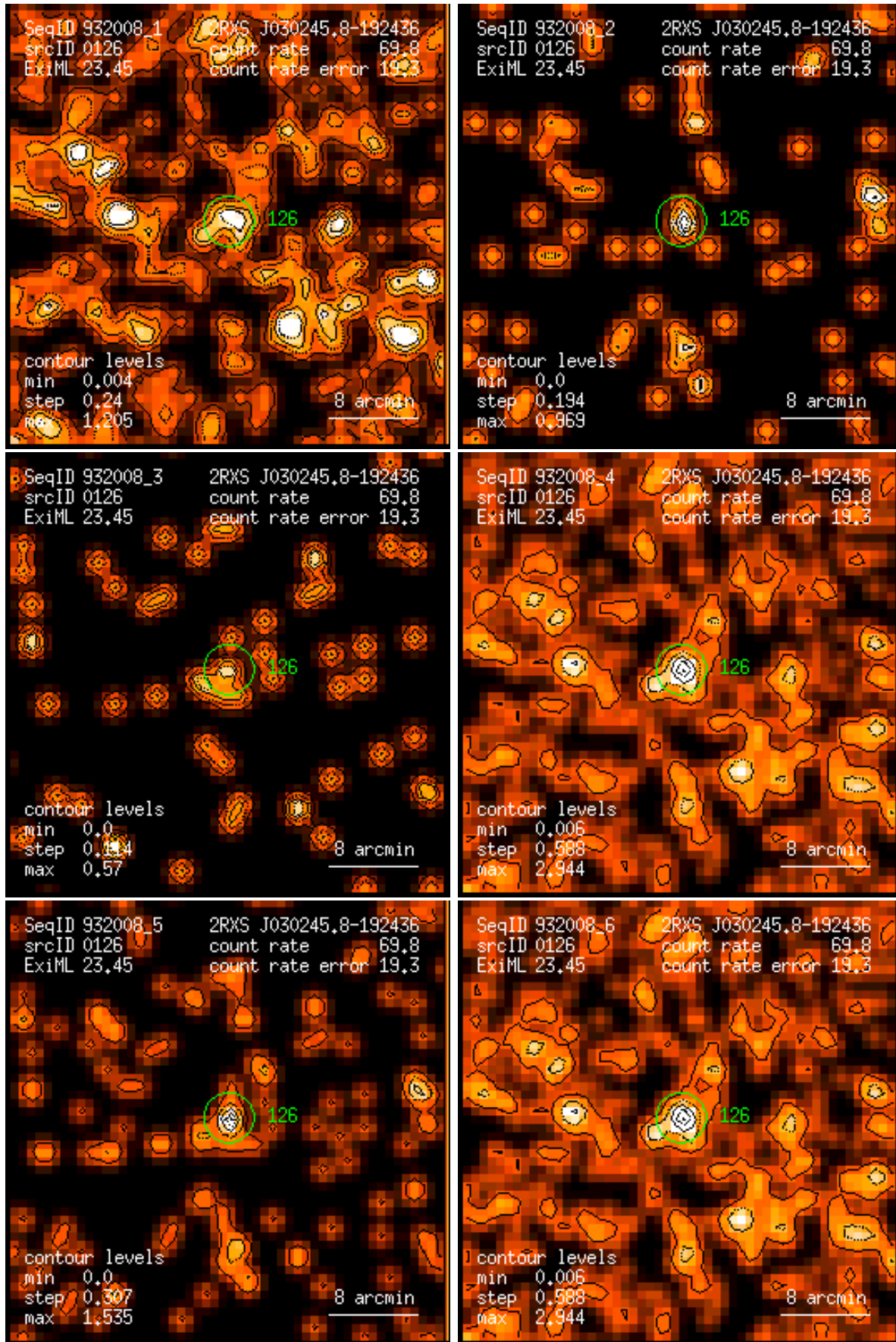
Figure 126: RASS 932008: detection 0126: band rate images, Gaussian filter: (1) PSPC channels 11 – 41, (2) 52 – 90, (3) 91 – 201, (4) 11 – 235, (5) 52 – 201, (6) 11 – 201. Broad band rates in counts/ks. Band rate contour levels in counts/ks/arcmin 2 .
