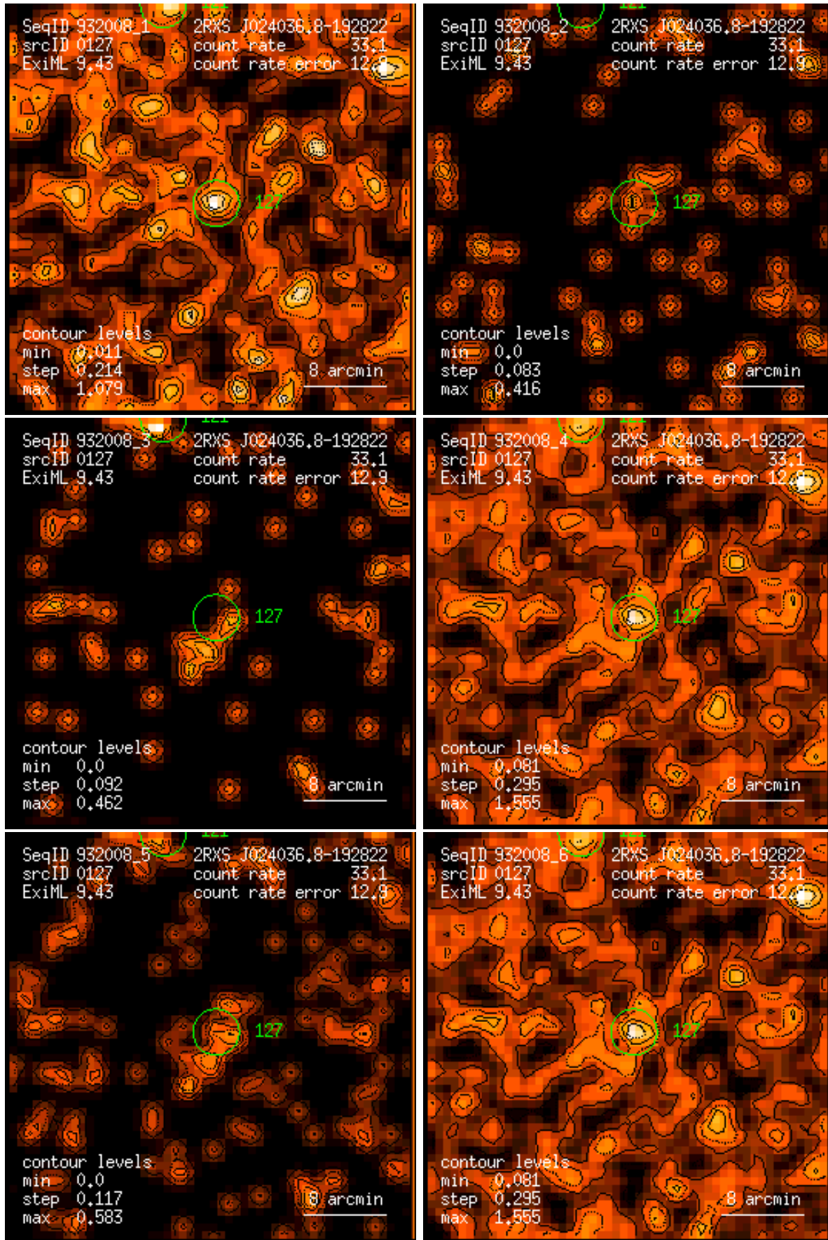
Figure 127: RASS 932008: detection 0127: band rate images, Gaussian filter: (1) PSPC channels 11 – 41, (2) 52 – 90, (3) 91 – 201, (4) 11 – 235, (5) 52 – 201, (6) 11 – 201. Broad band rates in counts/ks. Band rate contour levels in counts/ks/arcmin 2 .
