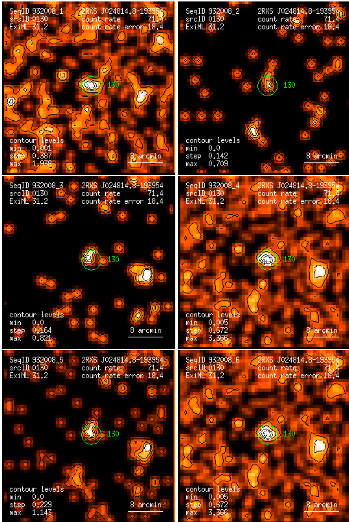
Figure 130: RASS 932008: detection 0130: band rate images, Gaussian filter: (1) PSPC channels 11 – 41, (2) 52 – 90, (3) 91 – 201, (4) 11 – 235, (5) 52 – 201, (6) 11 – 201. Broad band rates in counts/ks. Band rate contour levels in counts/ks/arcmin 2 .
