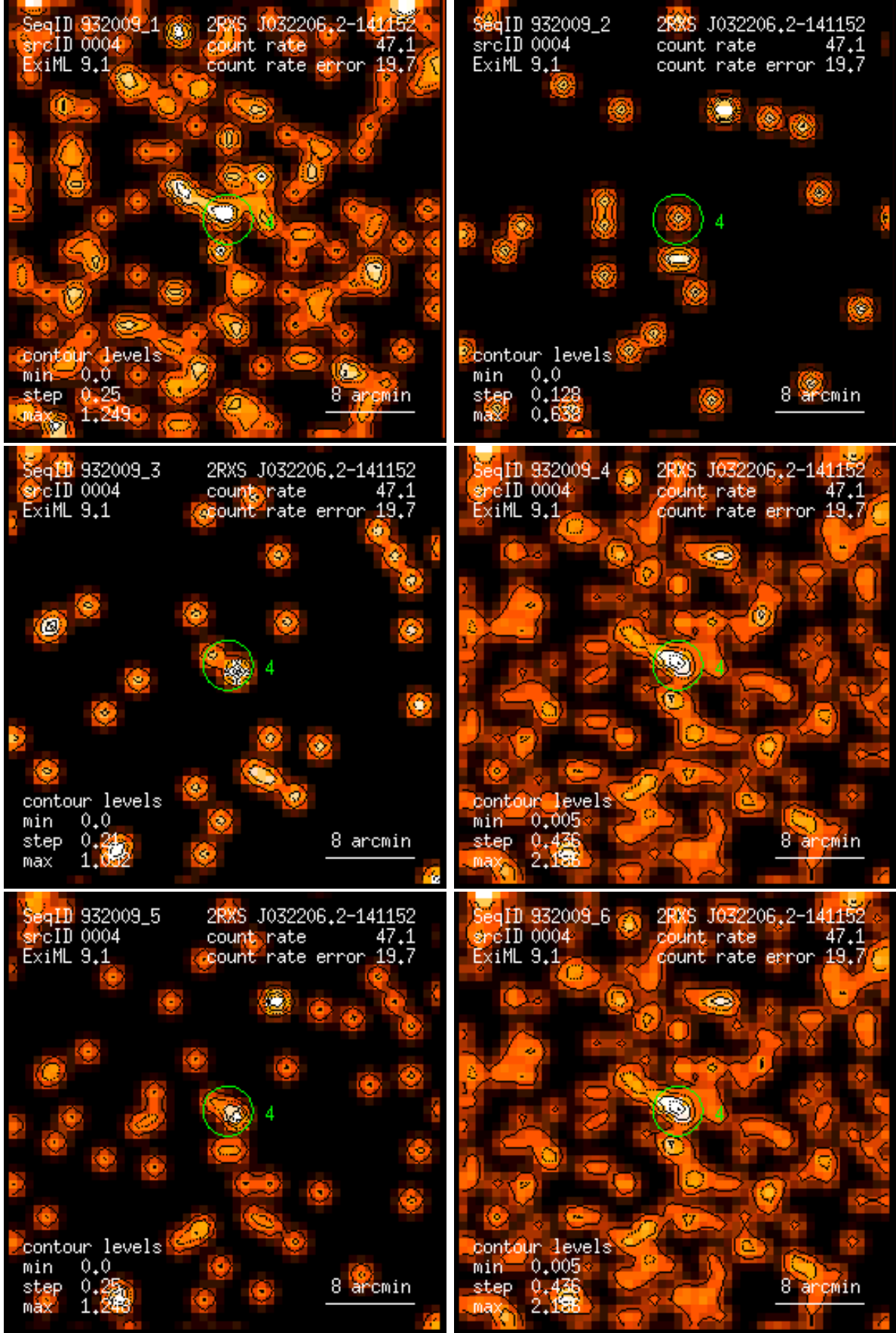
Figure 4: RASS 932009: detection 0004: band rate images, Gaussian filter: (1) PSPC channels 11 – 41, (2) 52 – 90, (3) 91 – 201, (4) 11 – 235, (5) 52 – 201, (6) 11 – 201. Broad band rates in counts/ks. Band rate contour levels in counts/ks/arcmin 2 .
