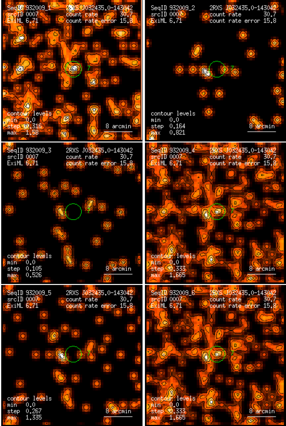
Figure 7: RASS 932009: detection 0007: band rate images, Gaussian filter: (1) PSPC channels 11 – 41, (2) 52 – 90, (3) 91 – 201, (4) 11 – 235, (5) 52 – 201, (6) 11 – 201. Broad band rates in counts/ks. Band rate contour levels in counts/ks/arcmin 2 .
