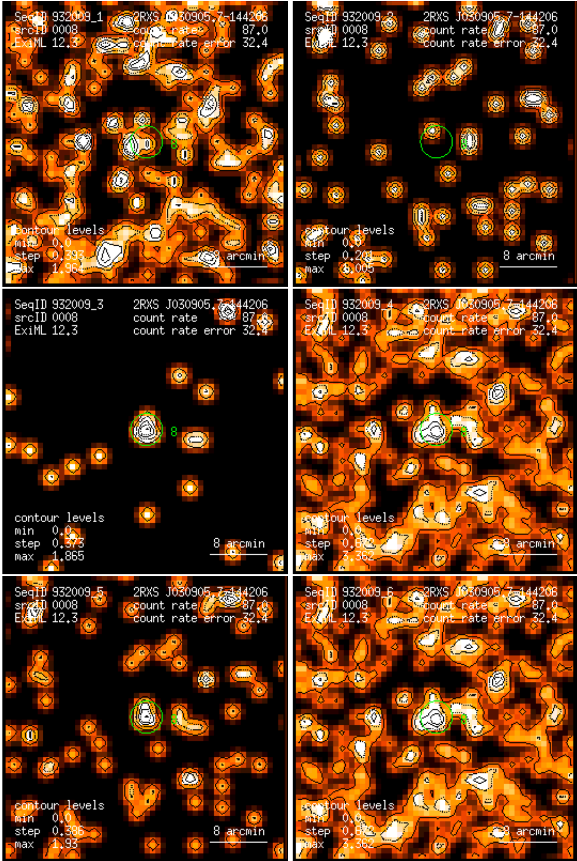
Figure 8: RASS 932009: detection 0008: band rate images, Gaussian filter: (1) PSPC channels 11 – 41, (2) 52 – 90, (3) 91 – 201, (4) 11 – 235, (5) 52 – 201, (6) 11 – 201. Broad band rates in counts/ks. Band rate contour levels in counts/ks/arcmin 2 .
