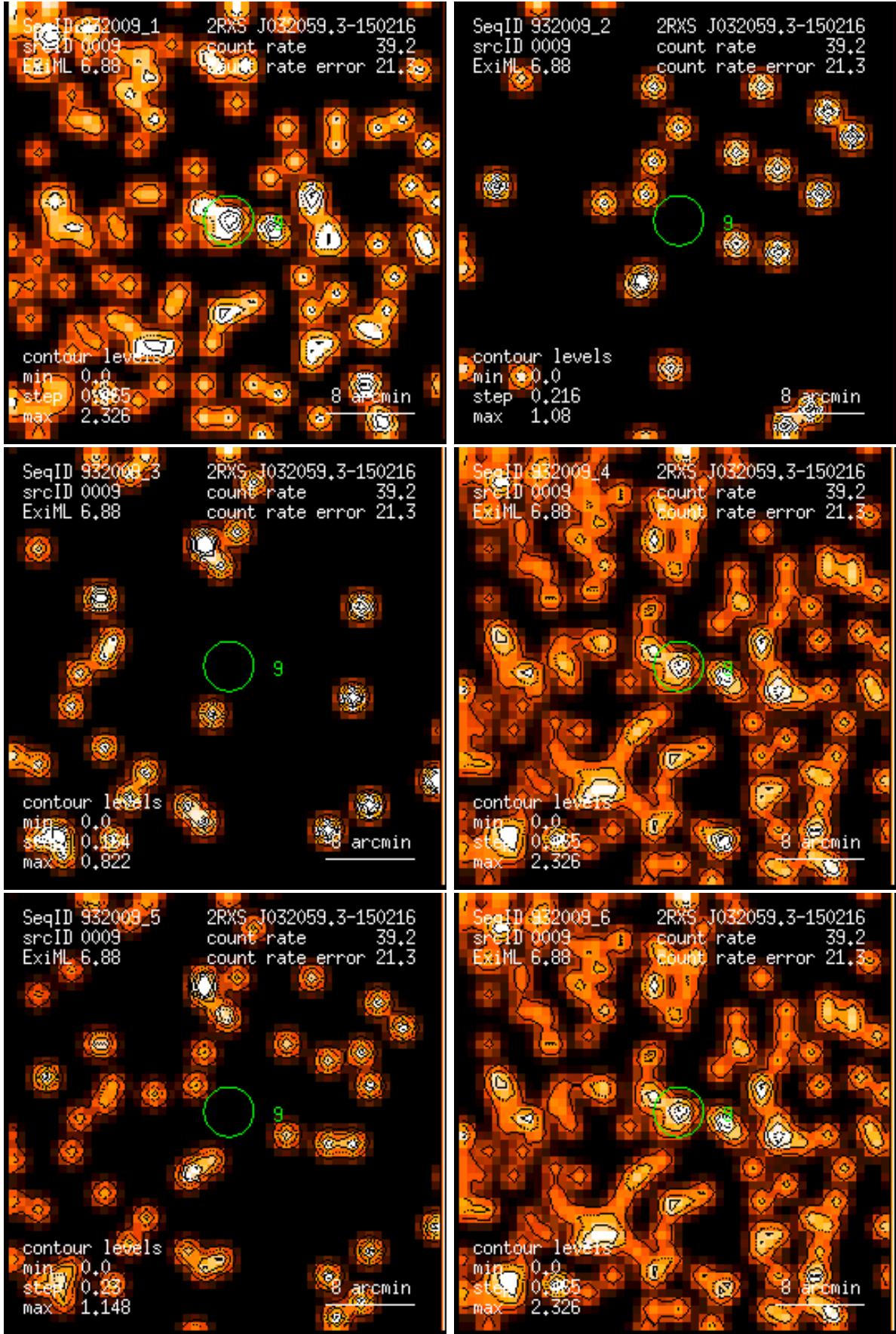
Figure 9: RASS 932009: detection 0009: band rate images, Gaussian filter: (1) PSPC channels 11 – 41, (2) 52 – 90, (3) 91 – 201, (4) 11 – 235, (5) 52 – 201, (6) 11 – 201. Broad band rates in counts/ks. Band rate contour levels in counts/ks/arcmin 2 .
