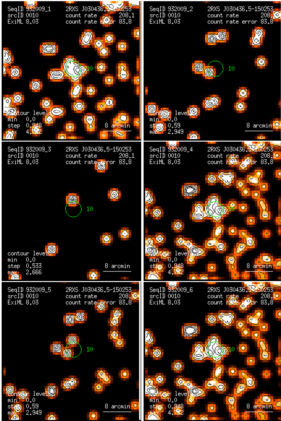
Figure 10: RASS 932009: detection 0010: band rate images, Gaussian filter: (1) PSPC channels 11 – 41, (2) 52 – 90, (3) 91 – 201, (4) 11 – 235, (5) 52 – 201, (6) 11 – 201. Broad band rates in counts/ks. Band rate contour levels in counts/ks/arcmin 2 .
