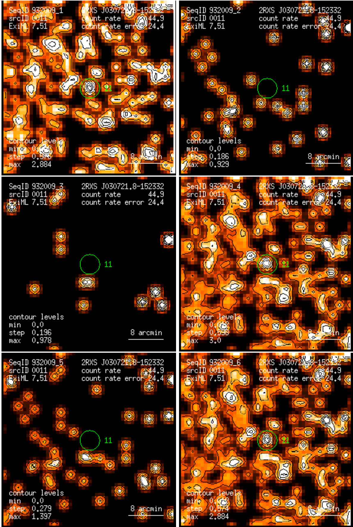
Figure 11: RASS 932009: detection 0011: band rate images, Gaussian filter: (1) PSPC channels 11 – 41, (2) 52 – 90, (3) 91 – 201, (4) 11 – 235, (5) 52 – 201, (6) 11 – 201. Broad band rates in counts/ks. Band rate contour levels in counts/ks/arcmin 2 .
