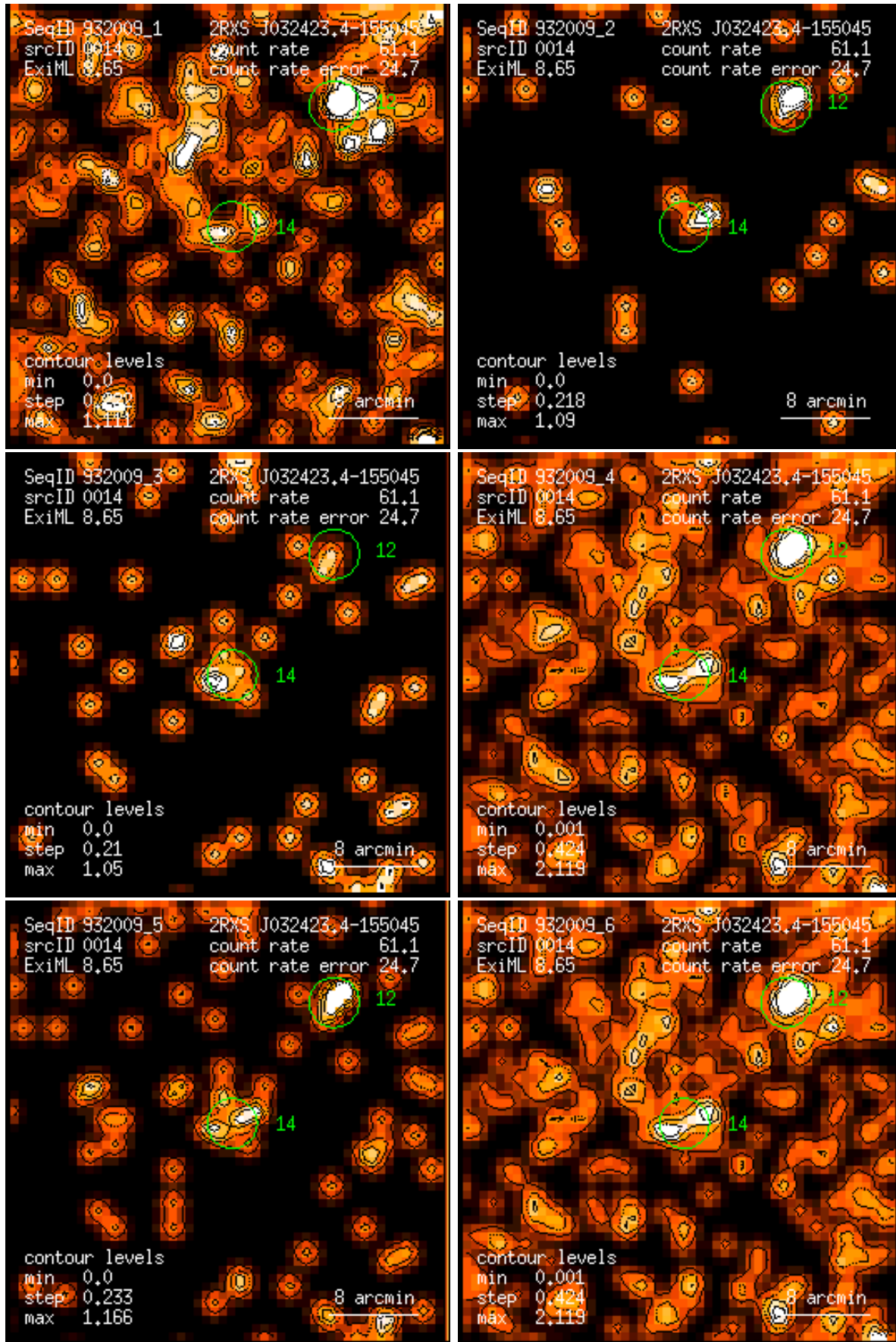
Figure 14: RASS 932009: detection 0014: band rate images, Gaussian filter: (1) PSPC channels 11 – 41, (2) 52 – 90, (3) 91 – 201, (4) 11 – 235, (5) 52 – 201, (6) 11 – 201. Broad band rates in counts/ks. Band rate contour levels in counts/ks/arcmin 2 .
