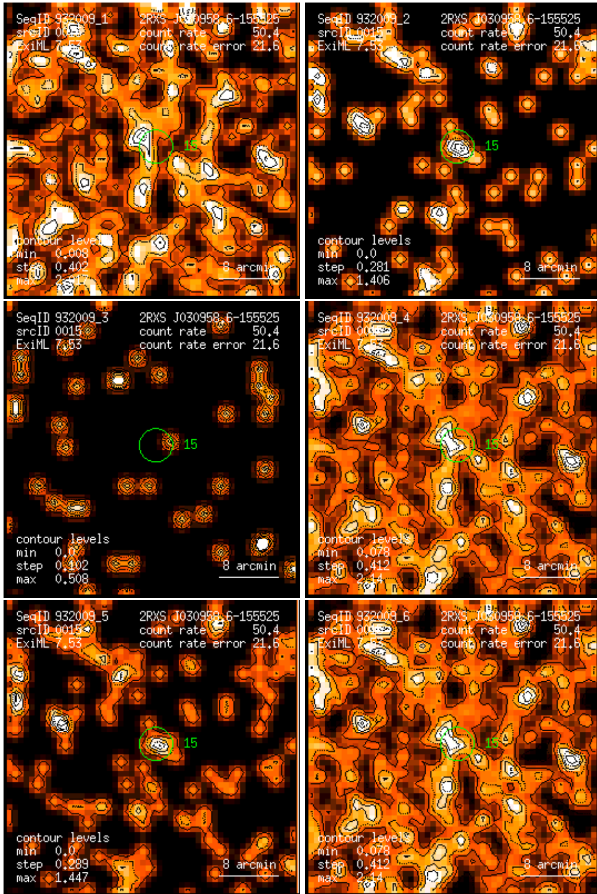
Figure 15: RASS 932009: detection 0015: band rate images, Gaussian filter: (1) PSPC channels 11 – 41, (2) 52 – 90, (3) 91 – 201, (4) 11 – 235, (5) 52 – 201, (6) 11 – 201. Broad band rates in counts/ks. Band rate contour levels in counts/ks/arcmin 2 .
