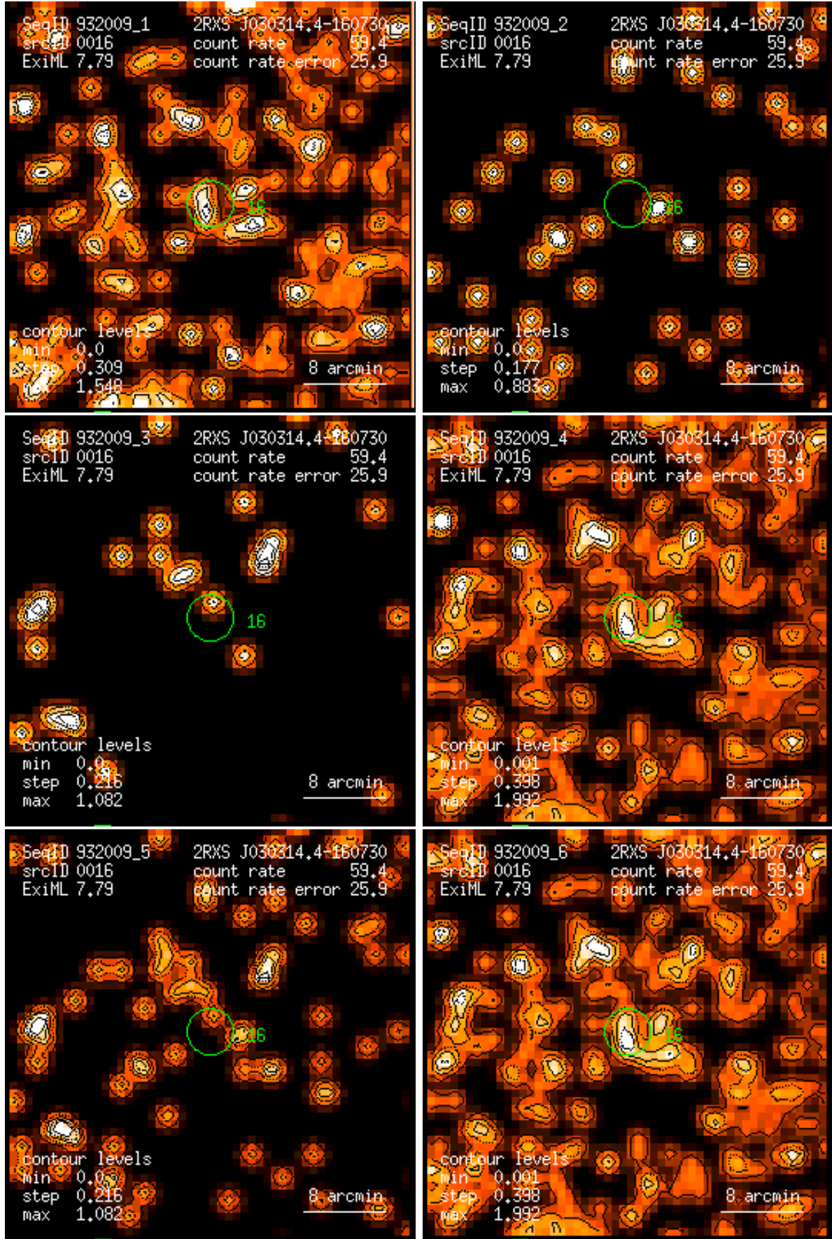
Figure 16: RASS 932009: detection 0016: band rate images, Gaussian filter: (1) PSPC channels 11 – 41, (2) 52 – 90, (3) 91 – 201, (4) 11 – 235, (5) 52 – 201, (6) 11 – 201. Broad band rates in counts/ks. Band rate contour levels in counts/ks/arcmin 2 .
