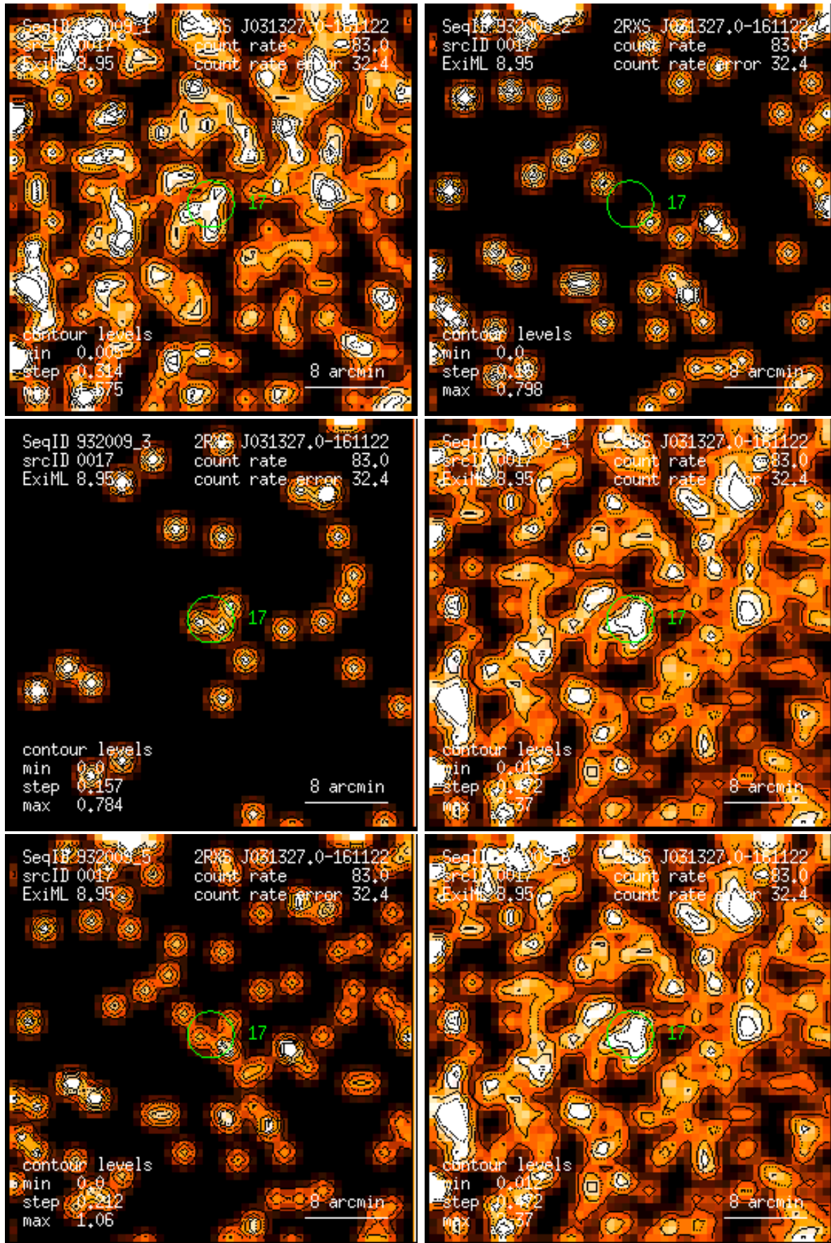
Figure 17: RASS 932009: detection 0017: band rate images, Gaussian filter: (1) PSPC channels 11 – 41, (2) 52 – 90, (3) 91 – 201, (4) 11 – 235, (5) 52 – 201, (6) 11 – 201. Broad band rates in counts/ks. Band rate contour levels in counts/ks/arcmin 2 .
