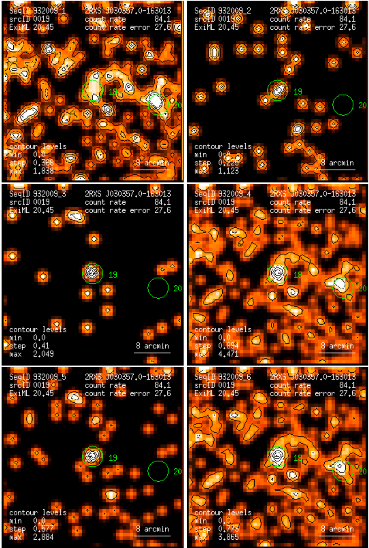
Figure 19: RASS 932009: detection 0019: band rate images, Gaussian filter: (1) PSPC channels 11 – 41, (2) 52 – 90, (3) 91 – 201, (4) 11 – 235, (5) 52 – 201, (6) 11 – 201. Broad band rates in counts/ks. Band rate contour levels in counts/ks/arcmin 2 .
